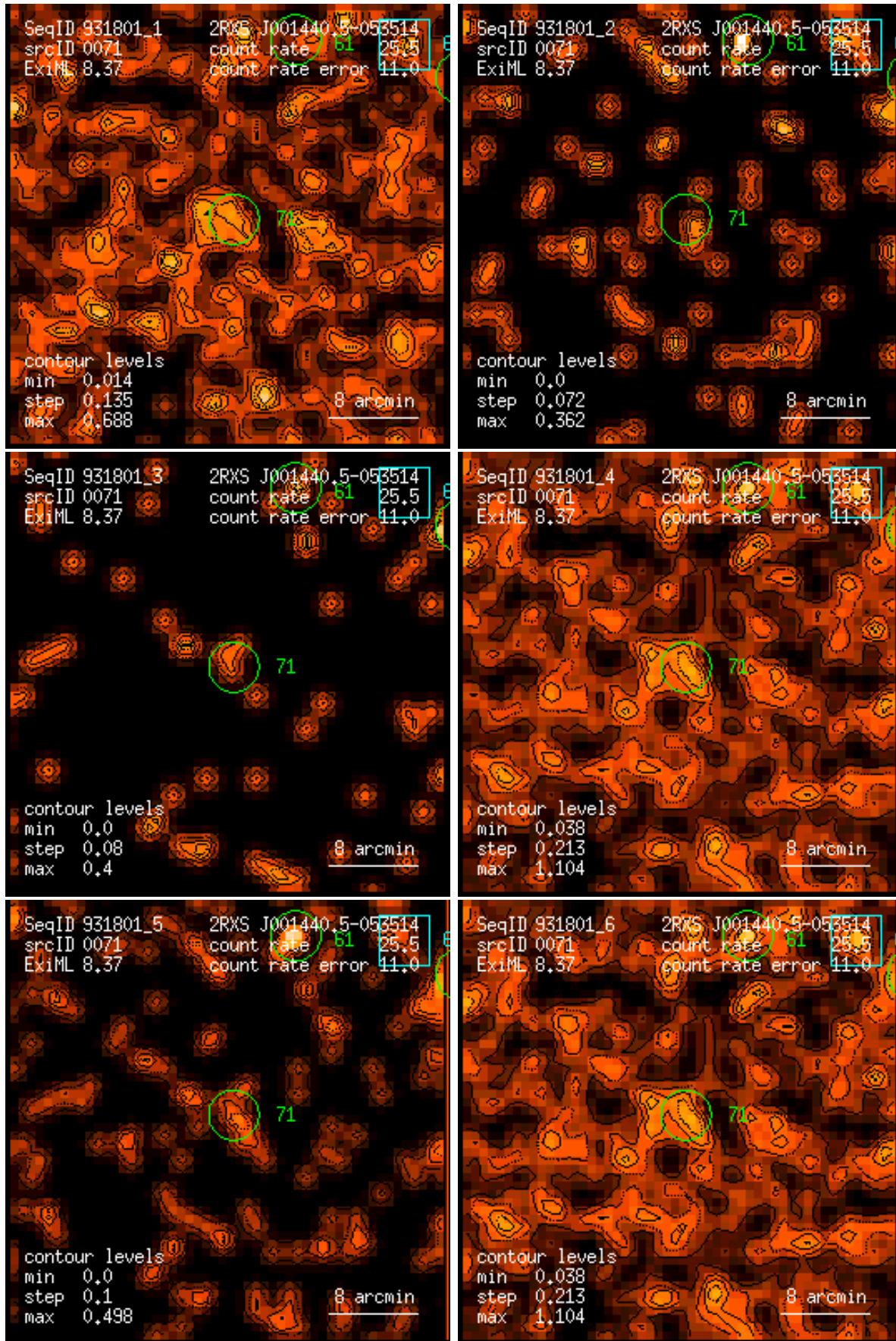
Figure 71: RASS 931801: detection 0071: band rate images, Gaussian filter: (1) PSPC channels 11 – 41, (2) 52 – 90, (3) 91 – 201, (4) 11 – 235, (5) 52 – 201, (6) 11 – 201. Broad band rates in counts/ks. Band rate contour levels in counts/ks/arcmin 2 .
