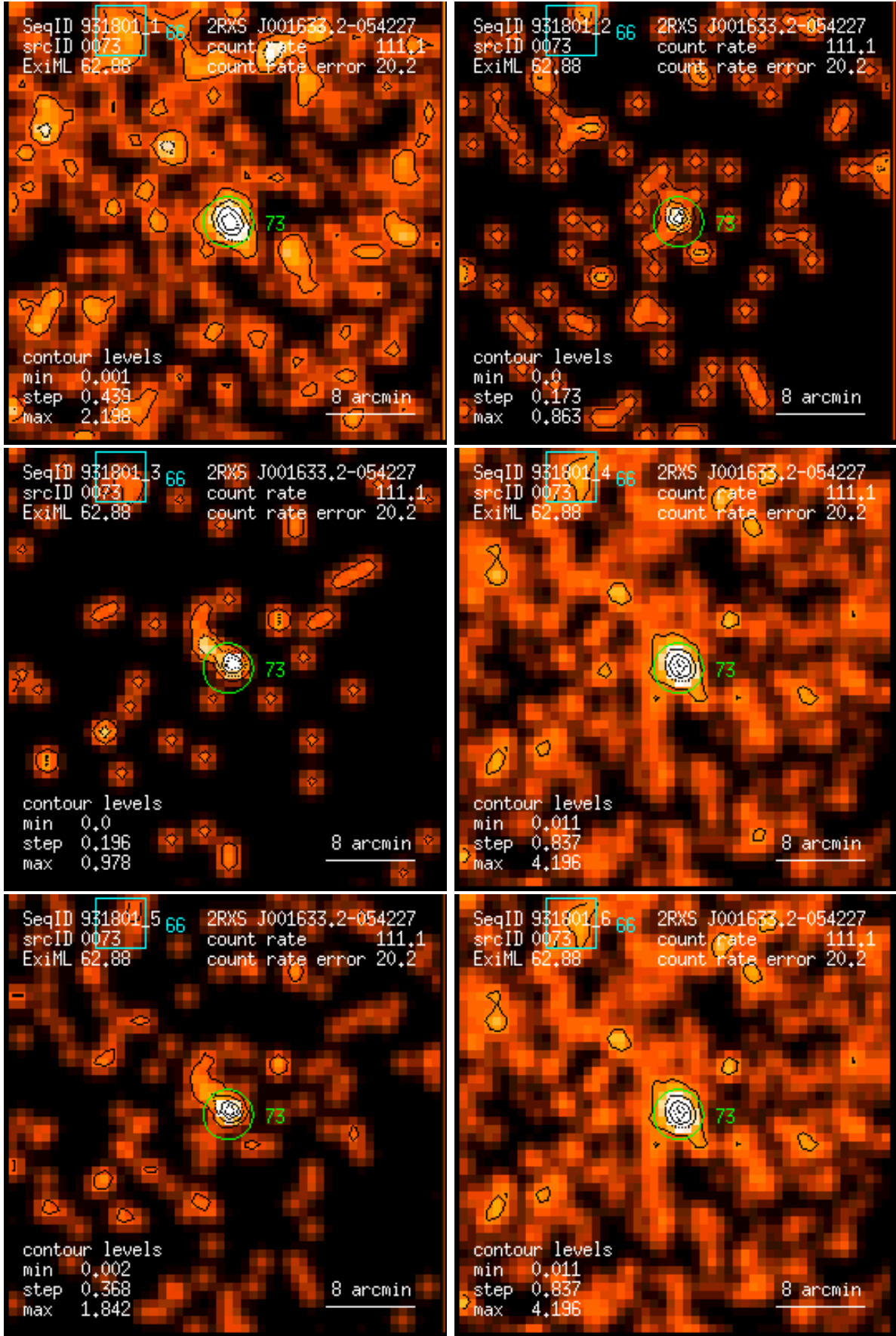
Figure 73: RASS 931801: detection 0073: band rate images, Gaussian filter: (1) PSPC channels 11 – 41, (2) 52 – 90, (3) 91 – 201, (4) 11 – 235, (5) 52 – 201, (6) 11 – 201. Broad band rates in counts/ks. Band rate contour levels in counts/ks/arcmin 2 .
