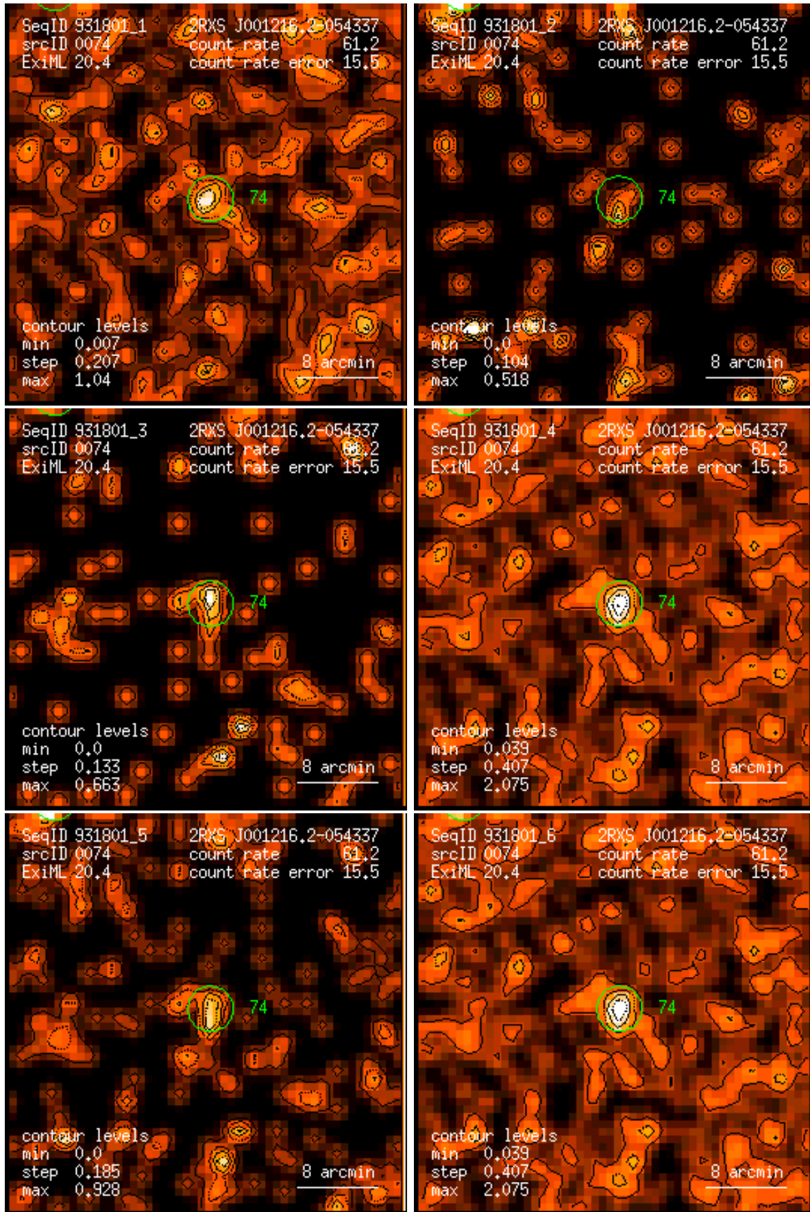
Figure 74: RASS 931801: detection 0074: band rate images, Gaussian filter: (1) PSPC channels 11 – 41, (2) 52 – 90, (3) 91 – 201, (4) 11 – 235, (5) 52 – 201, (6) 11 – 201. Broad band rates in counts/ks. Band rate contour levels in counts/ks/arcmin 2 .
