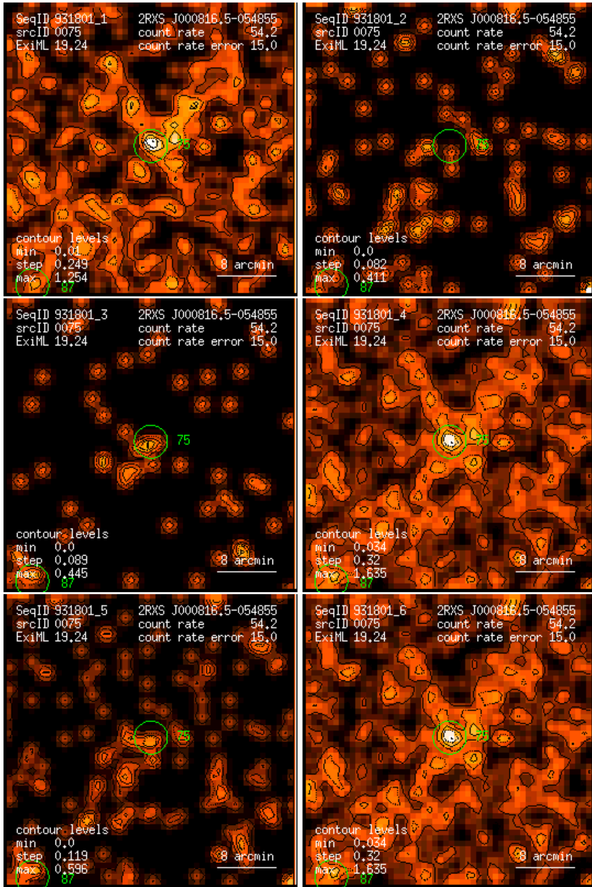
Figure 75: RASS 931801: detection 0075: band rate images, Gaussian filter: (1) PSPC channels 11 – 41, (2) 52 – 90, (3) 91 – 201, (4) 11 – 235, (5) 52 – 201, (6) 11 – 201. Broad band rates in counts/ks. Band rate contour levels in counts/ks/arcmin 2 .
