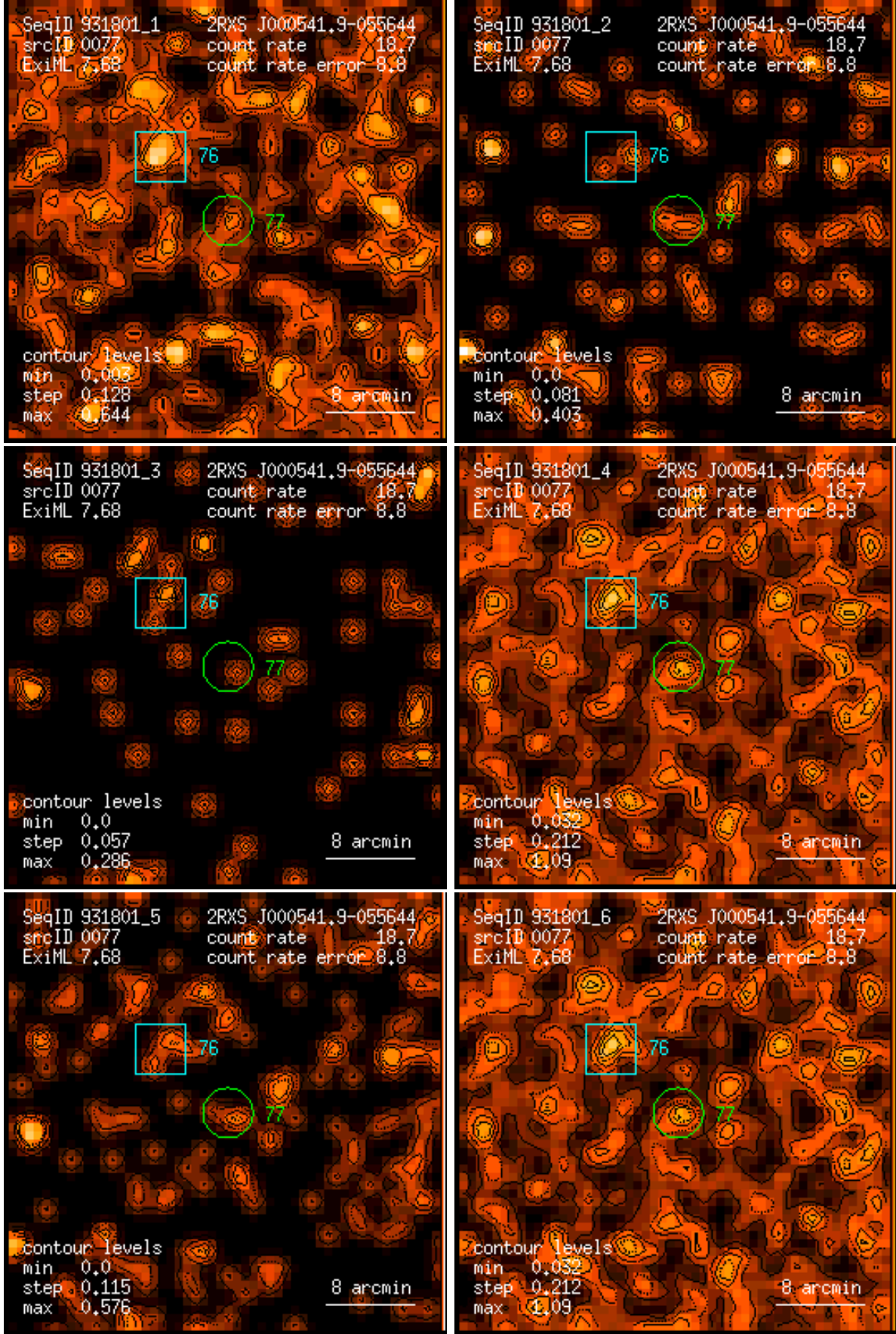
Figure 77: RASS 931801: detection 0077: band rate images, Gaussian filter: (1) PSPC channels 11 – 41, (2) 52 – 90, (3) 91 – 201, (4) 11 – 235, (5) 52 – 201, (6) 11 – 201. Broad band rates in counts/ks. Band rate contour levels in counts/ks/arcmin 2 .
