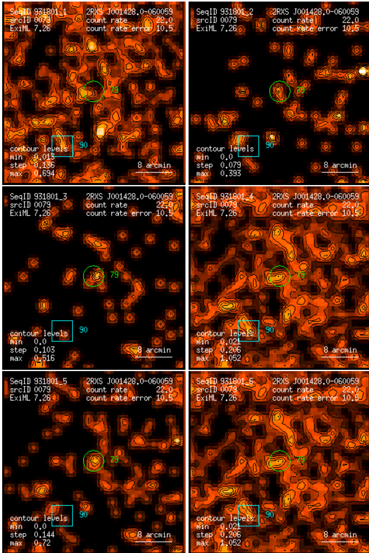
Figure 79: RASS 931801: detection 0079: band rate images, Gaussian filter: (1) PSPC channels 11 – 41, (2) 52 – 90, (3) 91 – 201, (4) 11 – 235, (5) 52 – 201, (6) 11 – 201. Broad band rates in counts/ks. Band rate contour levels in counts/ks/arcmin 2 .
