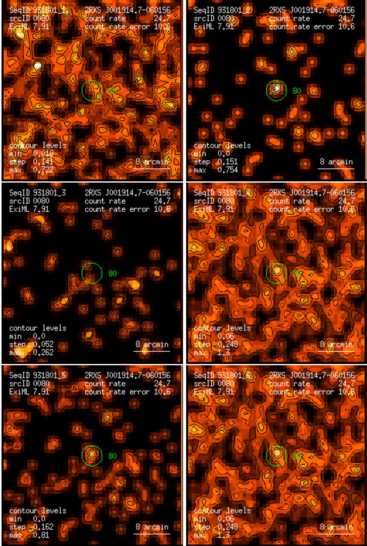
Figure 80: RASS 931801: detection 0080: band rate images, Gaussian filter: (1) PSPC channels 11 – 41, (2) 52 – 90, (3) 91 – 201, (4) 11 – 235, (5) 52 – 201, (6) 11 – 201. Broad band rates in counts/ks. Band rate contour levels in counts/ks/arcmin 2 .
