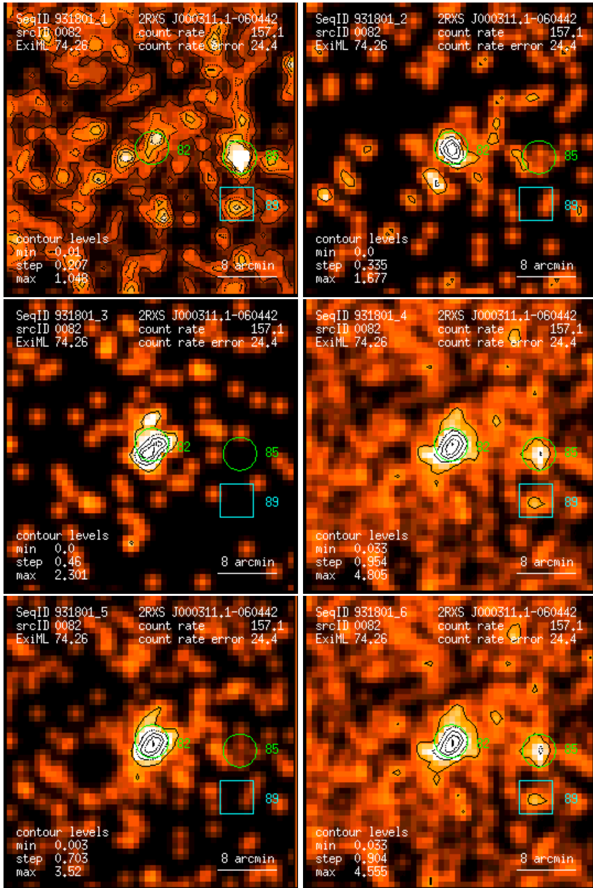
Figure 82: RASS 931801: detection 0082: band rate images, Gaussian filter: (1) PSPC channels 11 – 41, (2) 52 – 90, (3) 91 – 201, (4) 11 – 235, (5) 52 – 201, (6) 11 – 201. Broad band rates in counts/ks. Band rate contour levels in counts/ks/arcmin 2 .
