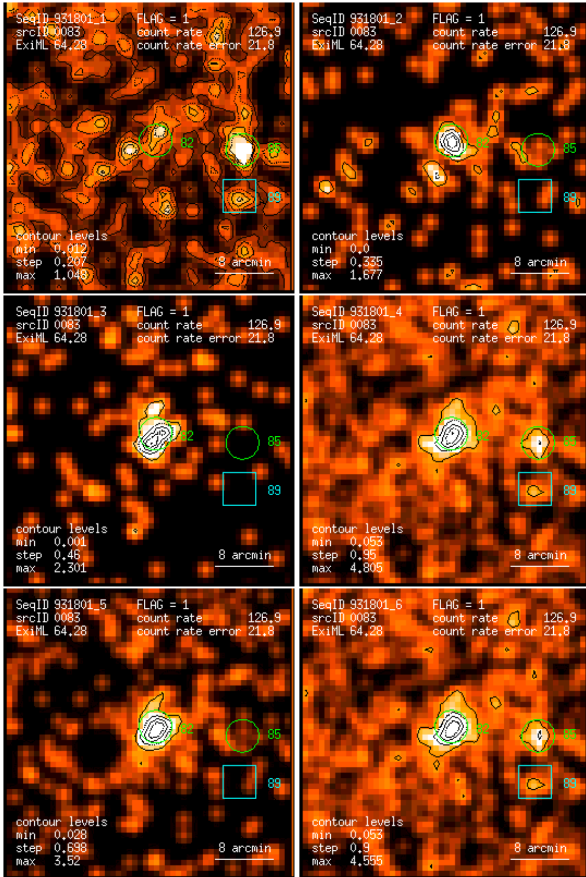
Figure 83: RASS 931801: detection 0083: band rate images, Gaussian filter: (1) PSPC channels 11 – 41, (2) 52 – 90, (3) 91 – 201, (4) 11 – 235, (5) 52 – 201, (6) 11 – 201. Broad band rates in counts/ks. Band rate contour levels in counts/ks/arcmin 2 .
