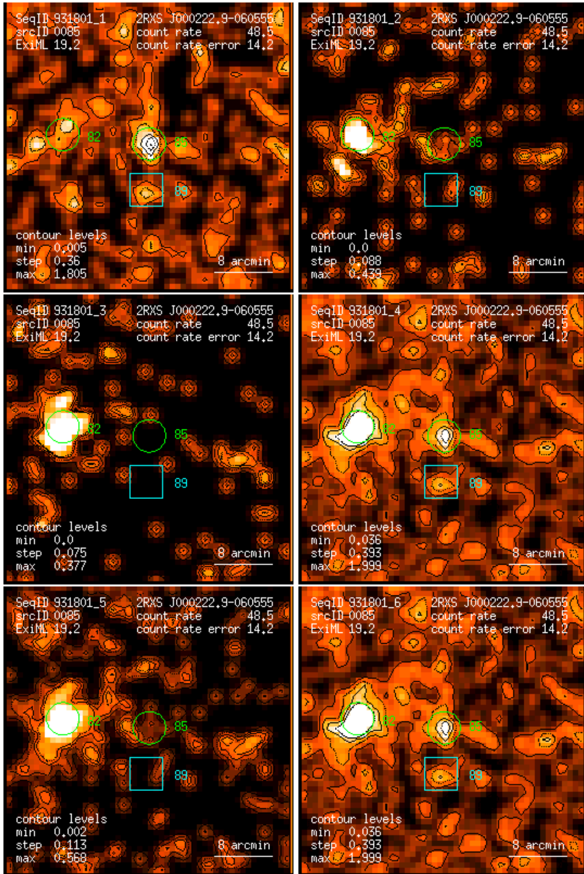
Figure 85: RASS 931801: detection 0085: band rate images, Gaussian filter: (1) PSPC channels 11 – 41, (2) 52 – 90, (3) 91 – 201, (4) 11 – 235, (5) 52 – 201, (6) 11 – 201. Broad band rates in counts/ks. Band rate contour levels in counts/ks/arcmin 2 .
