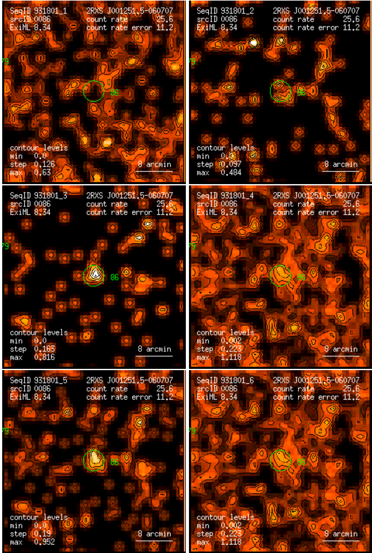
Figure 86: RASS 931801: detection 0086: band rate images, Gaussian filter: (1) PSPC channels 11 – 41, (2) 52 – 90, (3) 91 – 201, (4) 11 – 235, (5) 52 – 201, (6) 11 – 201. Broad band rates in counts/ks. Band rate contour levels in counts/ks/arcmin 2 .
