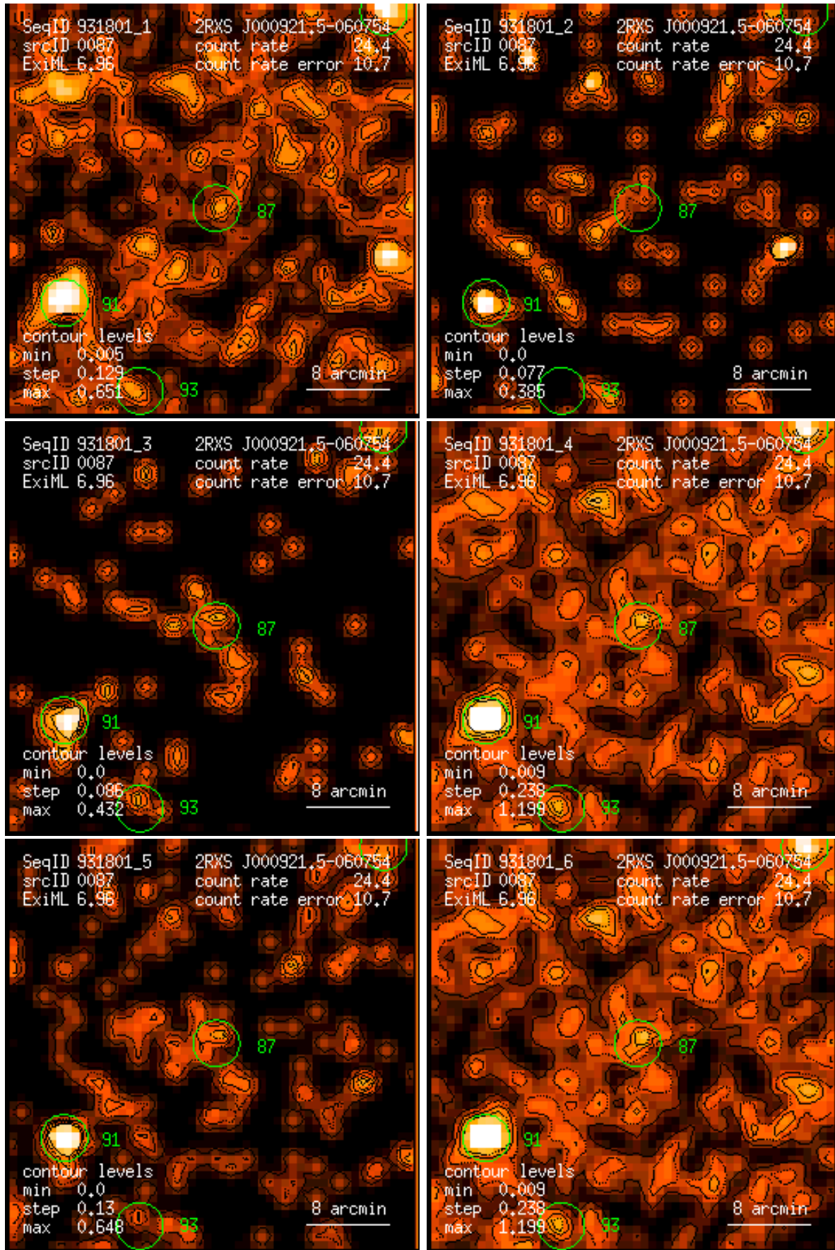
Figure 87: RASS 931801: detection 0087: band rate images, Gaussian filter: (1) PSPC channels 11 – 41, (2) 52 – 90, (3) 91 – 201, (4) 11 – 235, (5) 52 – 201, (6) 11 – 201. Broad band rates in counts/ks. Band rate contour levels in counts/ks/arcmin 2 .
