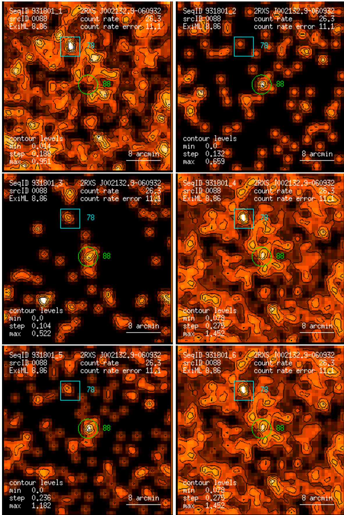
Figure 88: RASS 931801: detection 0088: band rate images, Gaussian filter: (1) PSPC channels 11 – 41, (2) 52 – 90, (3) 91 – 201, (4) 11 – 235, (5) 52 – 201, (6) 11 – 201. Broad band rates in counts/ks. Band rate contour levels in counts/ks/arcmin 2 .
