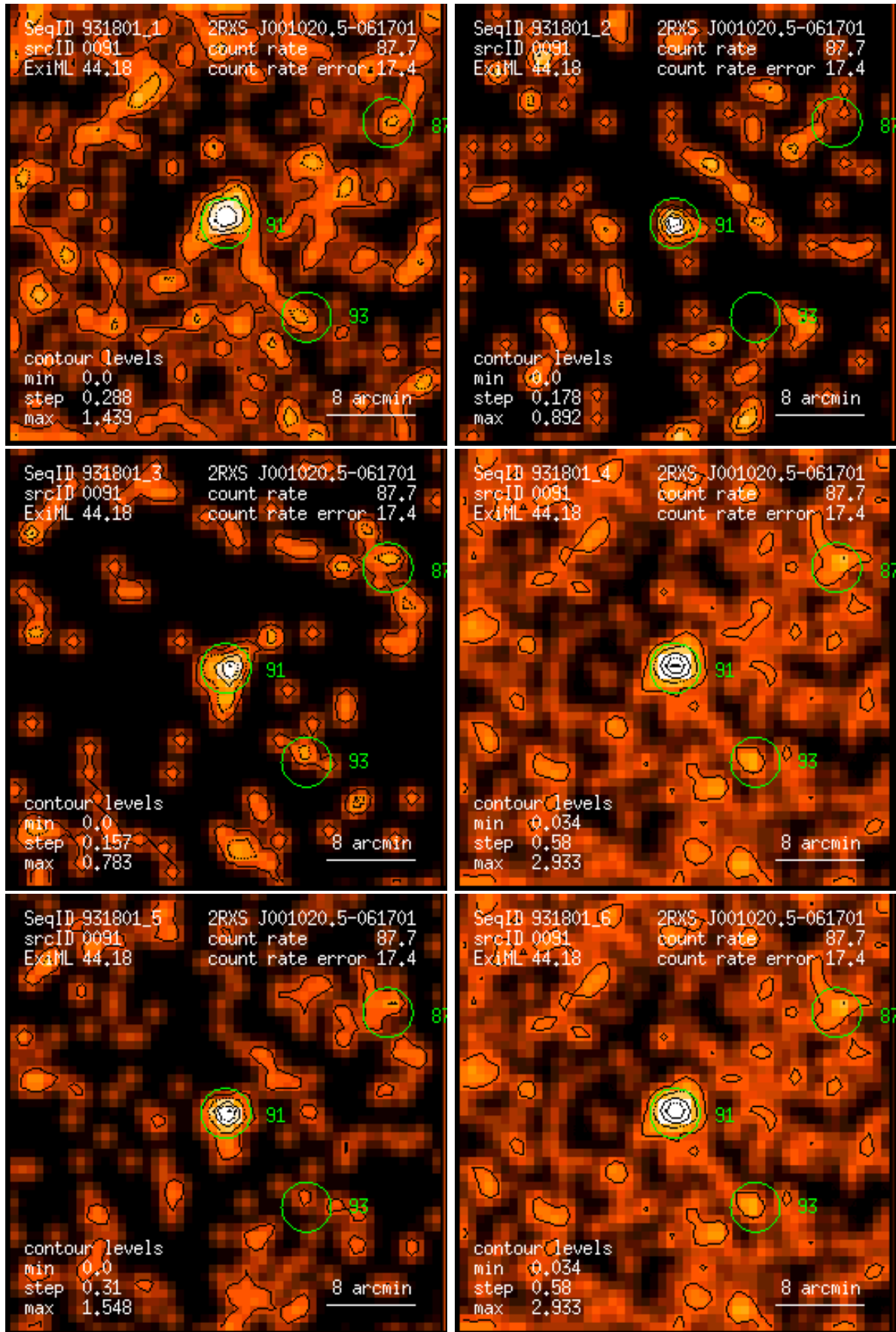
Figure 91: RASS 931801: detection 0091: band rate images, Gaussian filter: (1) PSPC channels 11 – 41, (2) 52 – 90, (3) 91 – 201, (4) 11 – 235, (5) 52 – 201, (6) 11 – 201. Broad band rates in counts/ks. Band rate contour levels in counts/ks/arcmin 2 .
