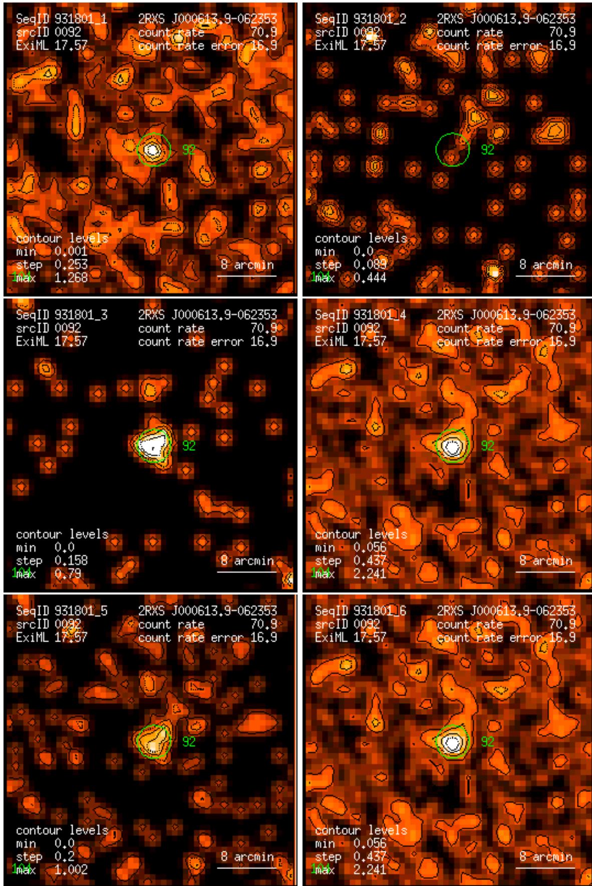
Figure 92: RASS 931801: detection 0092: band rate images, Gaussian filter: (1) PSPC channels 11 – 41, (2) 52 – 90, (3) 91 – 201, (4) 11 – 235, (5) 52 – 201, (6) 11 – 201. Broad band rates in counts/ks. Band rate contour levels in counts/ks/arcmin 2 .
