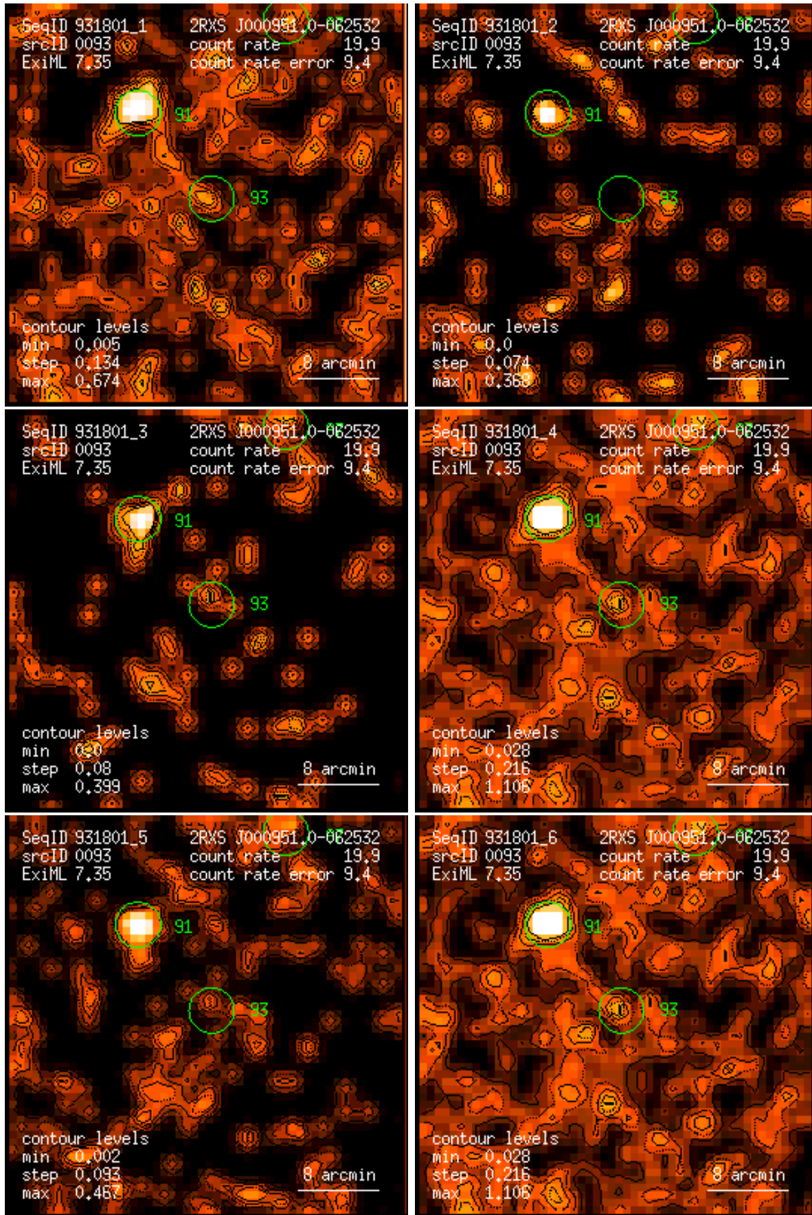
Figure 93: RASS 931801: detection 0093: band rate images, Gaussian filter: (1) PSPC channels 11 – 41, (2) 52 – 90, (3) 91 – 201, (4) 11 – 235, (5) 52 – 201, (6) 11 – 201. Broad band rates in counts/ks. Band rate contour levels in counts/ks/arcmin 2 .
