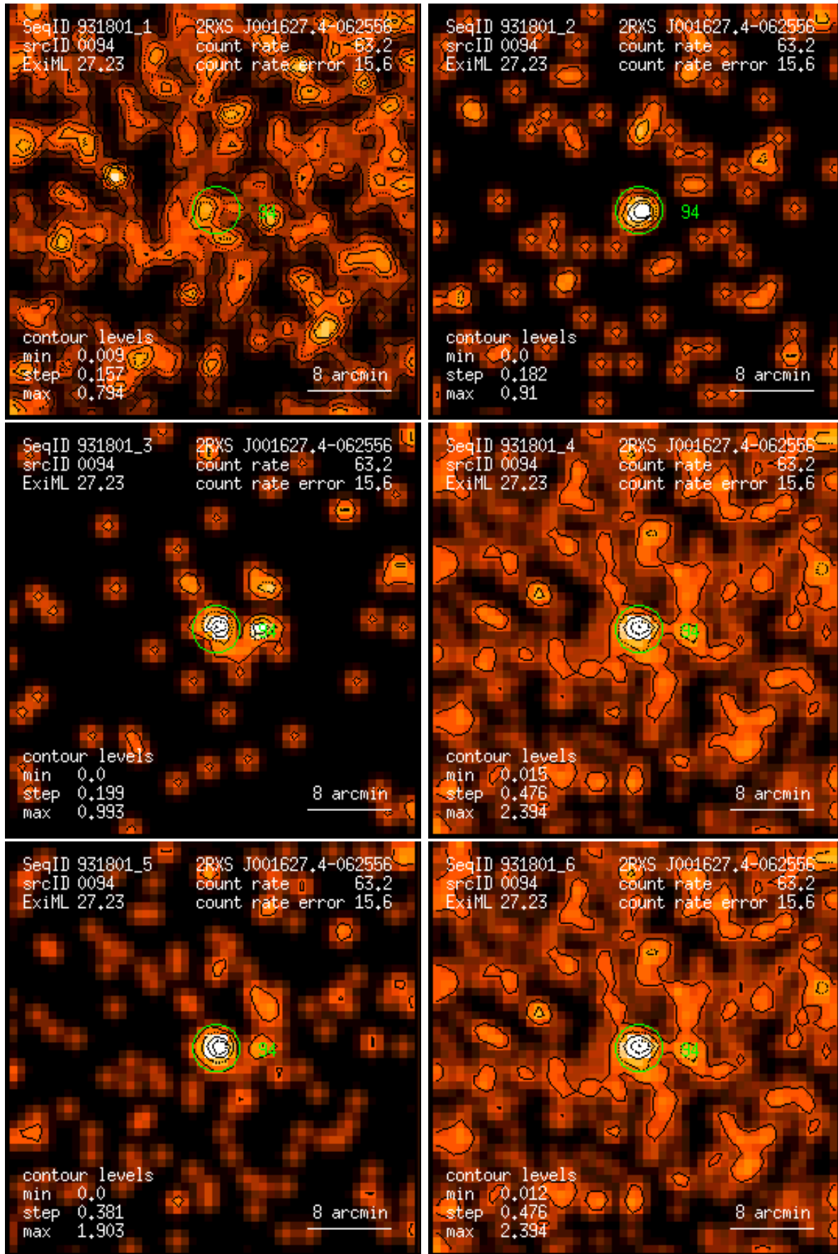
Figure 94: RASS 931801: detection 0094: band rate images, Gaussian filter: (1) PSPC channels 11 – 41, (2) 52 – 90, (3) 91 – 201, (4) 11 – 235, (5) 52 – 201, (6) 11 – 201. Broad band rates in counts/ks. Band rate contour levels in counts/ks/arcmin 2 .
