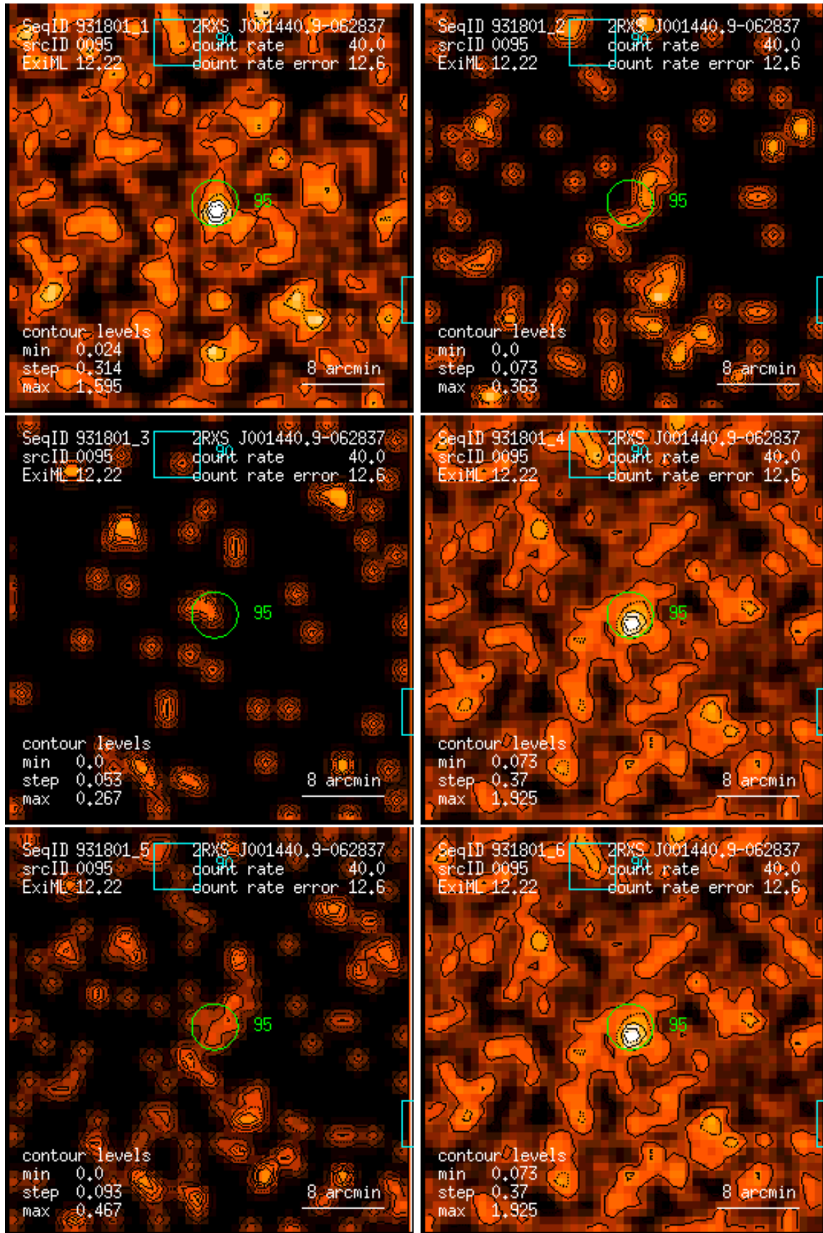
Figure 95: RASS 931801: detection 0095: band rate images, Gaussian filter: (1) PSPC channels 11 – 41, (2) 52 – 90, (3) 91 – 201, (4) 11 – 235, (5) 52 – 201, (6) 11 – 201. Broad band rates in counts/ks. Band rate contour levels in counts/ks/arcmin 2 .
