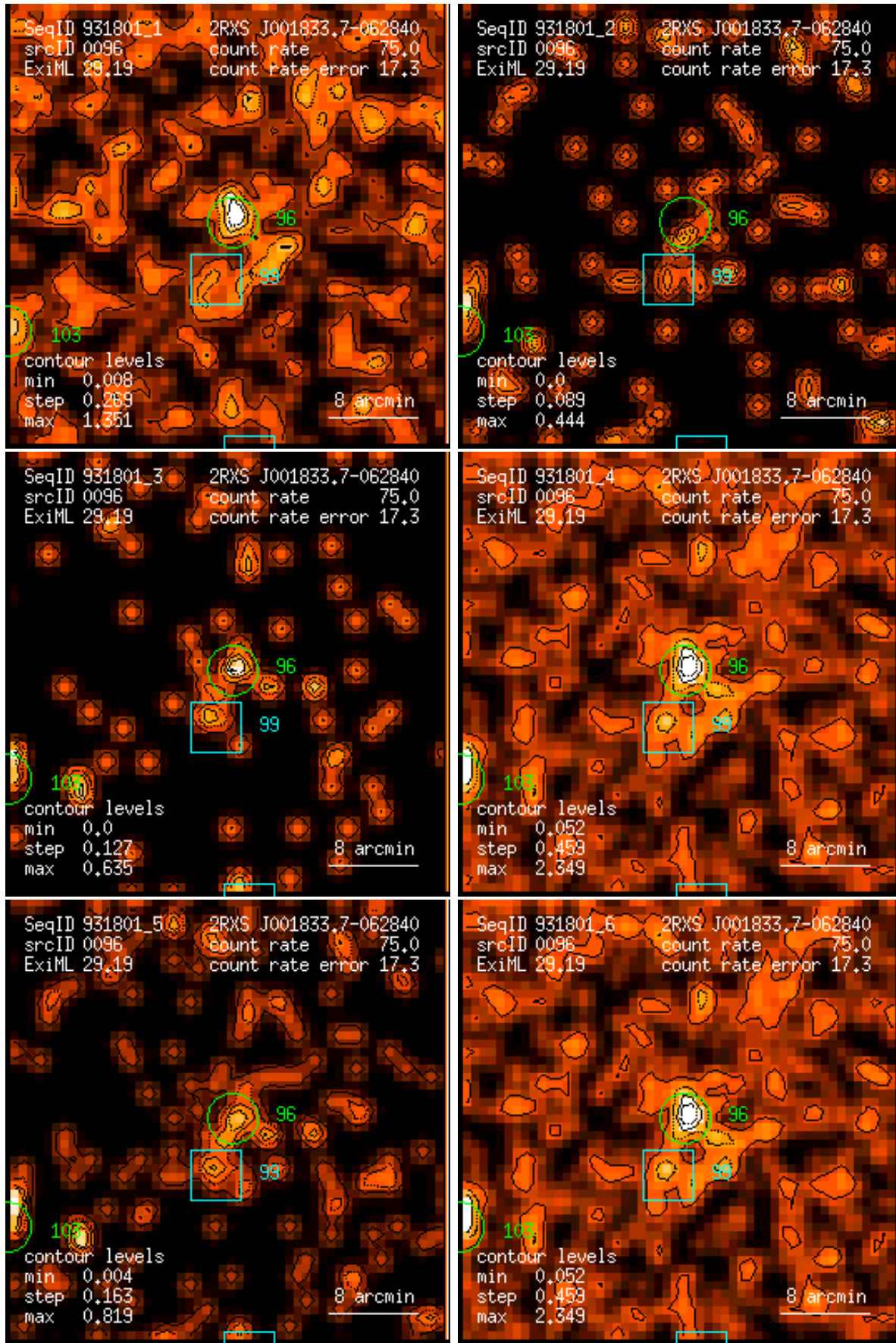
Figure 96: RASS 931801: detection 0096: band rate images, Gaussian filter: (1) PSPC channels 11 – 41, (2) 52 – 90, (3) 91 – 201, (4) 11 – 235, (5) 52 – 201, (6) 11 – 201. Broad band rates in counts/ks. Band rate contour levels in counts/ks/arcmin 2 .
