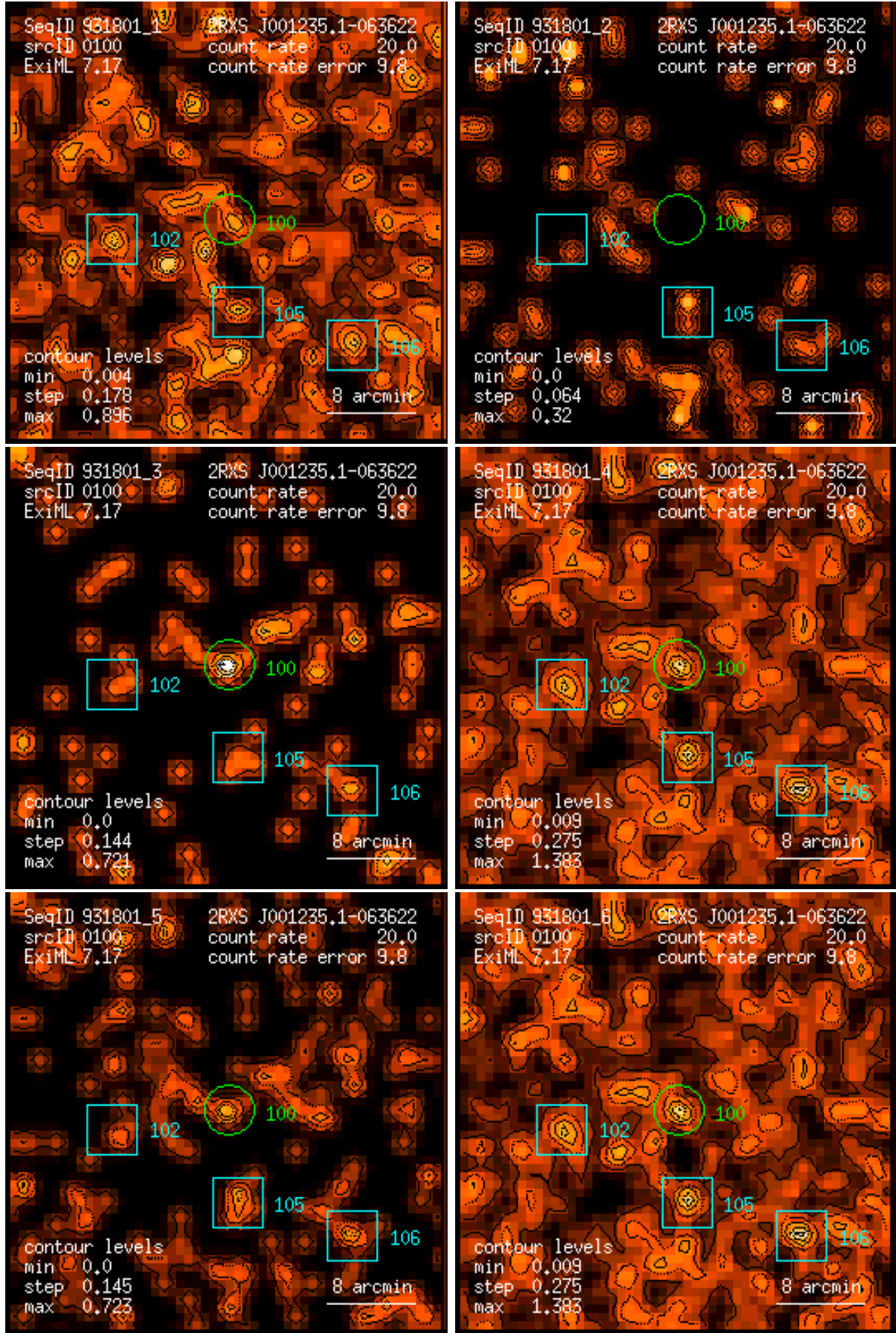
Figure 100: RASS 931801: detection 0100: band rate images, Gaussian filter: (1) PSPC channels 11 – 41, (2) 52 – 90, (3) 91 – 201, (4) 11 – 235, (5) 52 – 201, (6) 11 – 201. Broad band rates in counts/ks. Band rate contour levels in counts/ks/arcmin 2 .
