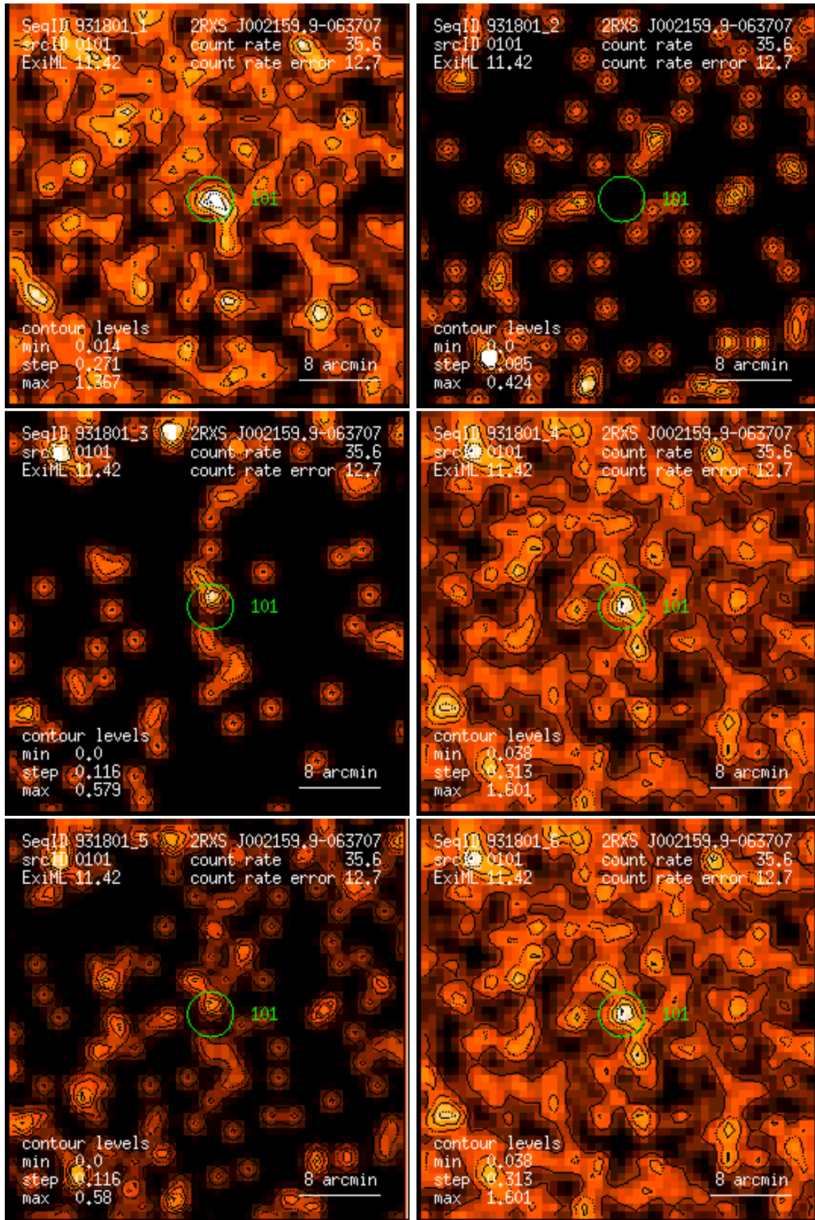
Figure 101: RASS 931801: detection 0101: band rate images, Gaussian filter: (1) PSPC channels 11 – 41, (2) 52 – 90, (3) 91 – 201, (4) 11 – 235, (5) 52 – 201, (6) 11 – 201. Broad band rates in counts/ks. Band rate contour levels in counts/ks/arcmin 2 .
