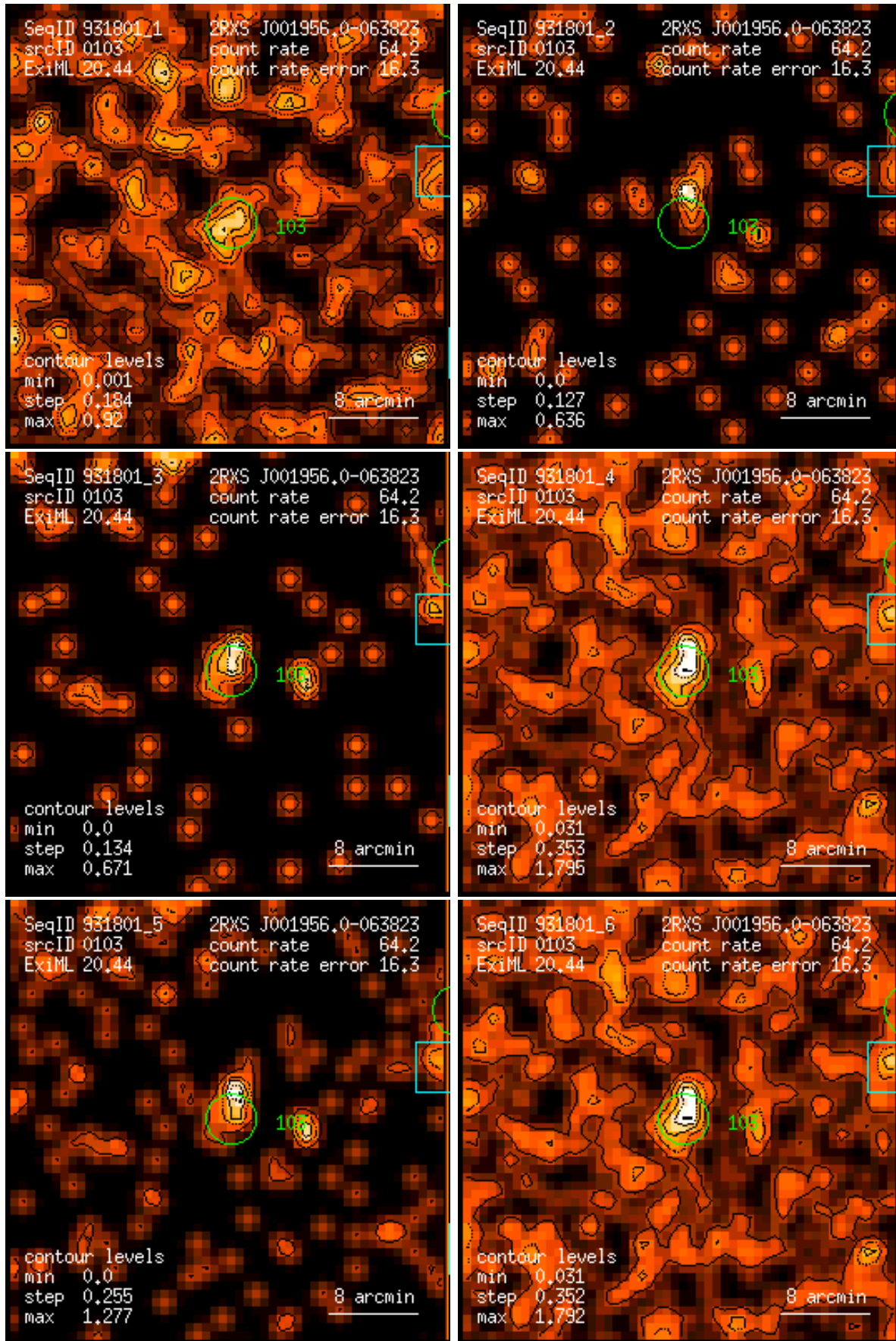
Figure 103: RASS 931801: detection 0103: band rate images, Gaussian filter: (1) PSPC channels 11 – 41, (2) 52 – 90, (3) 91 – 201, (4) 11 – 235, (5) 52 – 201, (6) 11 – 201. Broad band rates in counts/ks. Band rate contour levels in counts/ks/arcmin 2 .
