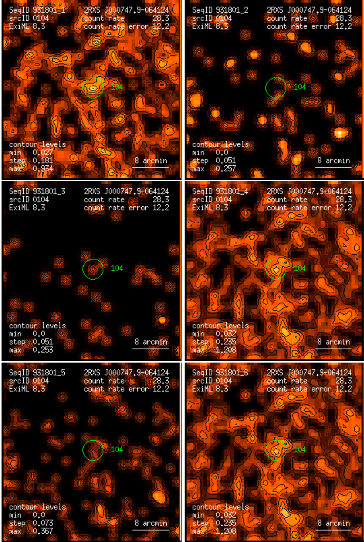
Figure 104: RASS 931801: detection 0104: band rate images, Gaussian filter: (1) PSPC channels 11 – 41, (2) 52 – 90, (3) 91 – 201, (4) 11 – 235, (5) 52 – 201, (6) 11 – 201. Broad band rates in counts/ks. Band rate contour levels in counts/ks/arcmin 2 .
