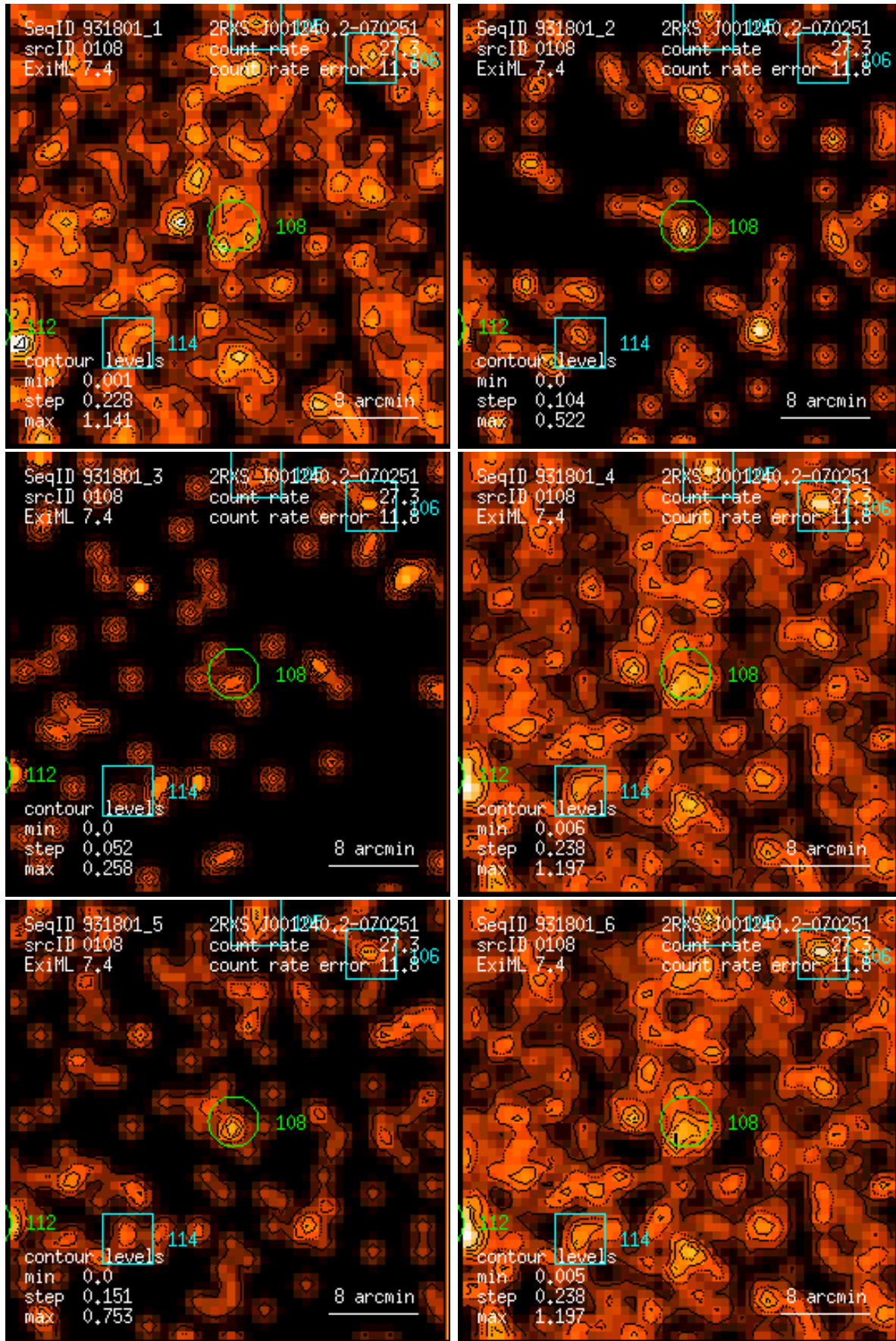
Figure 108: RASS 931801: detection 0108: band rate images, Gaussian filter: (1) PSPC channels 11 – 41, (2) 52 – 90, (3) 91 – 201, (4) 11 – 235, (5) 52 – 201, (6) 11 – 201. Broad band rates in counts/ks. Band rate contour levels in counts/ks/arcmin 2 .
