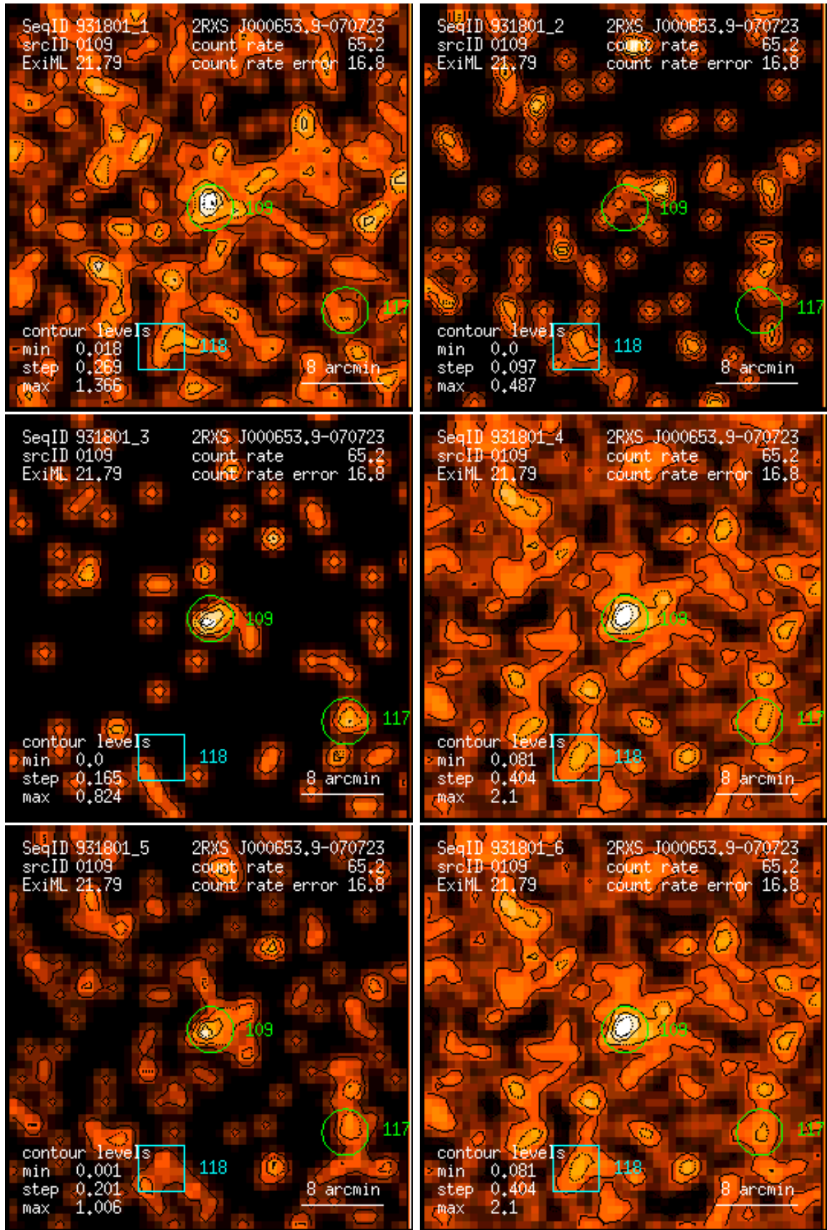
Figure 109: RASS 931801: detection 0109: band rate images, Gaussian filter: (1) PSPC channels 11 – 41, (2) 52 – 90, (3) 91 – 201, (4) 11 – 235, (5) 52 – 201, (6) 11 – 201. Broad band rates in counts/ks. Band rate contour levels in counts/ks/arcmin 2 .
