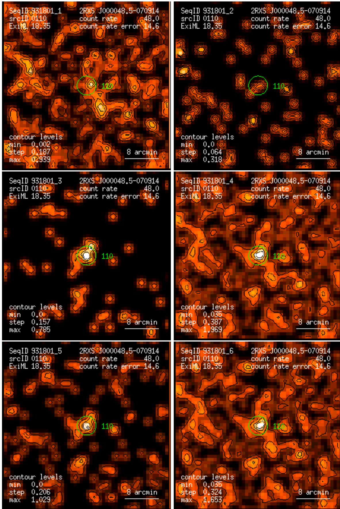
Figure 110: RASS 931801: detection 0110: band rate images, Gaussian filter: (1) PSPC channels 11 – 41, (2) 52 – 90, (3) 91 – 201, (4) 11 – 235, (5) 52 – 201, (6) 11 – 201. Broad band rates in counts/ks. Band rate contour levels in counts/ks/arcmin 2 .
