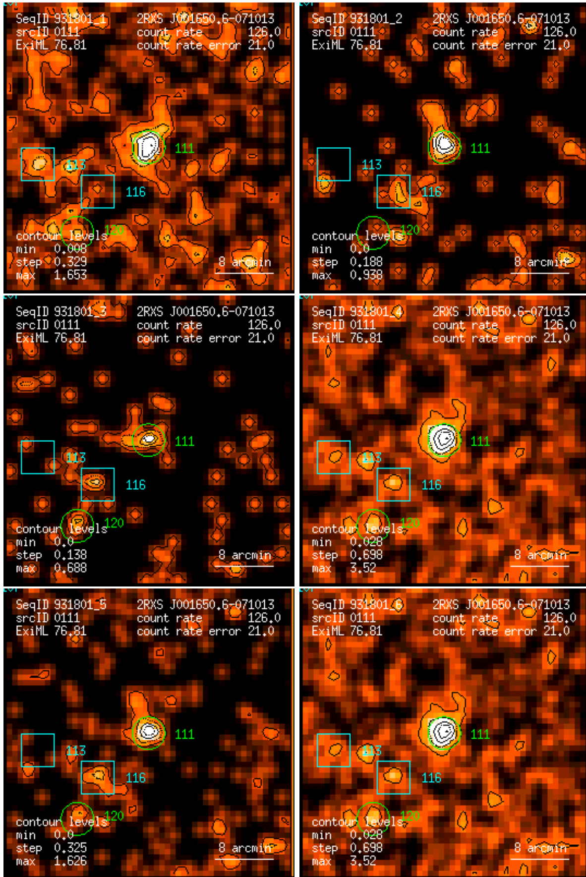
Figure 111: RASS 931801: detection 0111: band rate images, Gaussian filter: (1) PSPC channels 11 – 41, (2) 52 – 90, (3) 91 – 201, (4) 11 – 235, (5) 52 – 201, (6) 11 – 201. Broad band rates in counts/ks. Band rate contour levels in counts/ks/arcmin 2 .
