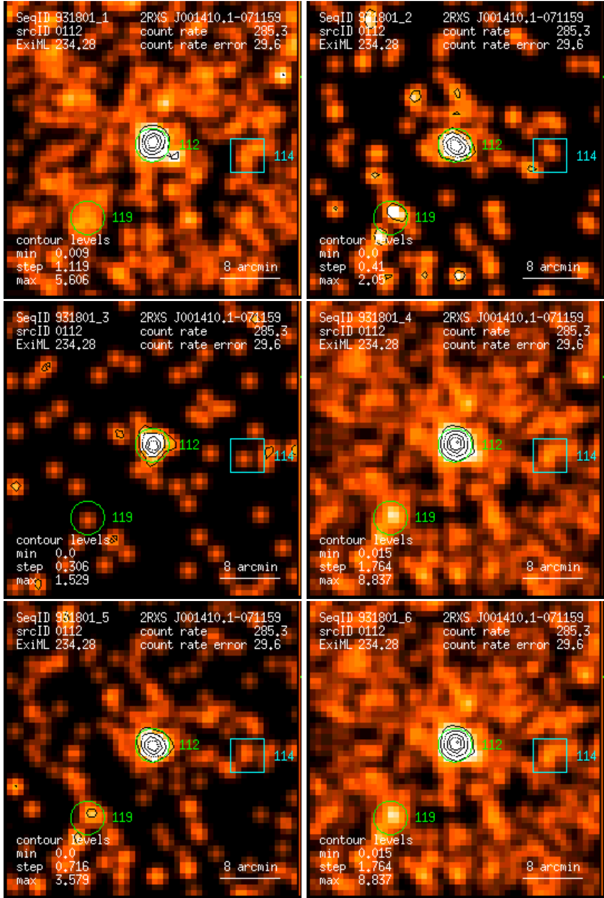
Figure 112: RASS 931801: detection 0112: band rate images, Gaussian filter: (1) PSPC channels 11 – 41, (2) 52 – 90, (3) 91 – 201, (4) 11 – 235, (5) 52 – 201, (6) 11 – 201. Broad band rates in counts/ks. Band rate contour levels in counts/ks/arcmin 2 .
