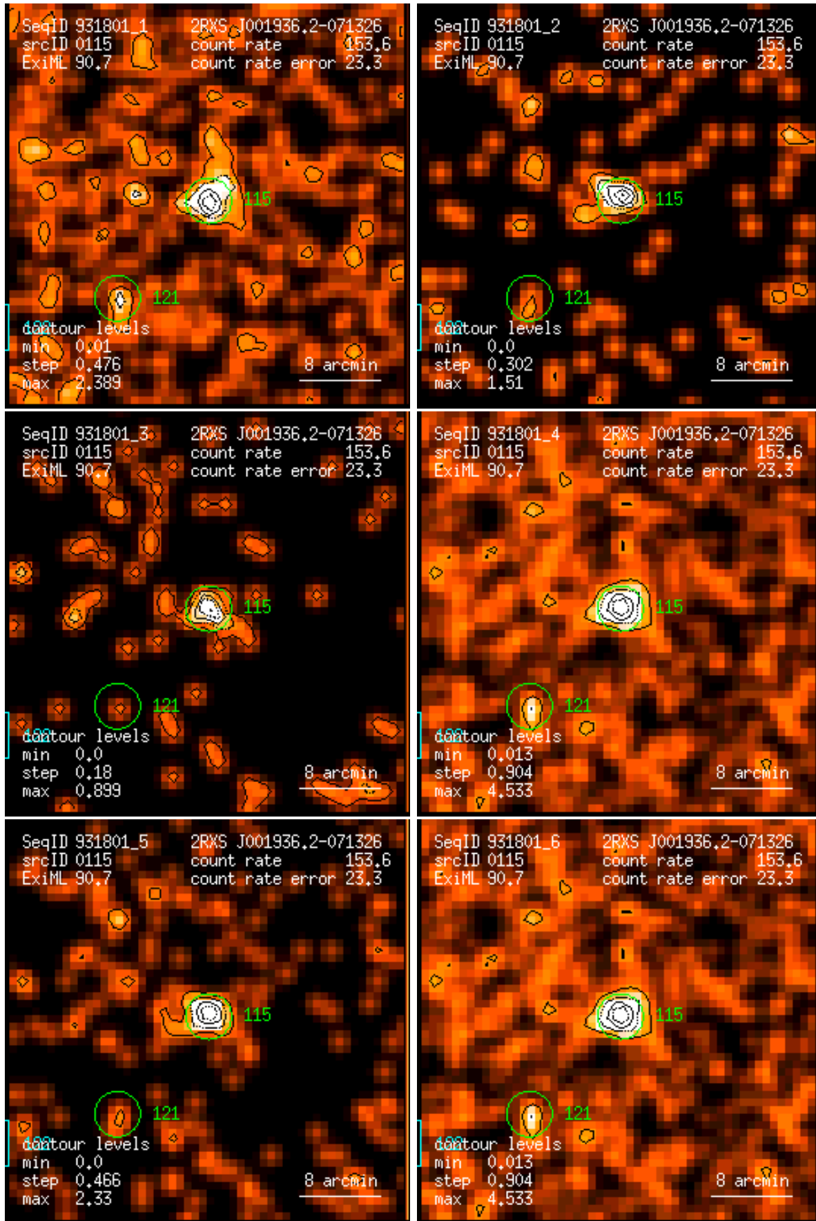
Figure 115: RASS 931801: detection 0115: band rate images, Gaussian filter: (1) PSPC channels 11 – 41, (2) 52 – 90, (3) 91 – 201, (4) 11 – 235, (5) 52 – 201, (6) 11 – 201. Broad band rates in counts/ks. Band rate contour levels in counts/ks/arcmin 2 .
