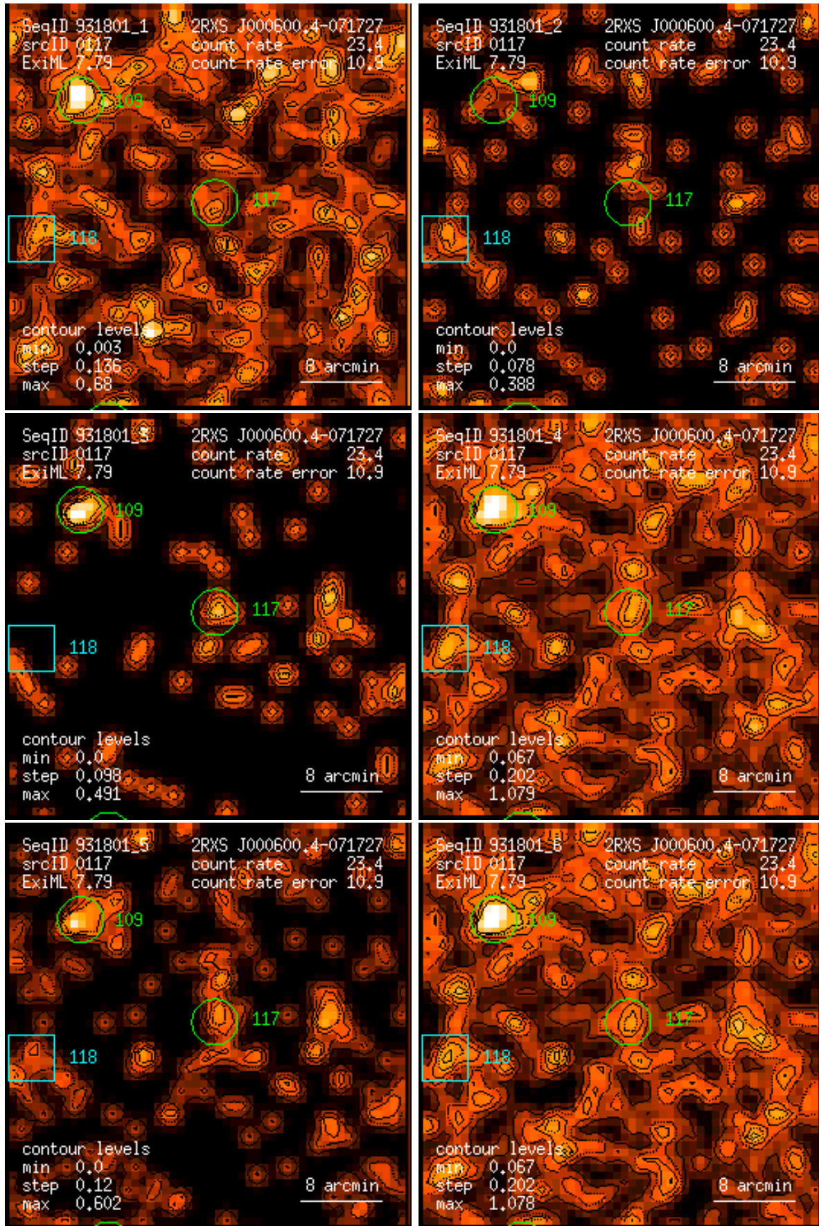
Figure 117: RASS 931801: detection 0117: band rate images, Gaussian filter: (1) PSPC channels 11 – 41, (2) 52 – 90, (3) 91 – 201, (4) 11 – 235, (5) 52 – 201, (6) 11 – 201. Broad band rates in counts/ks. Band rate contour levels in counts/ks/arcmin 2 .
