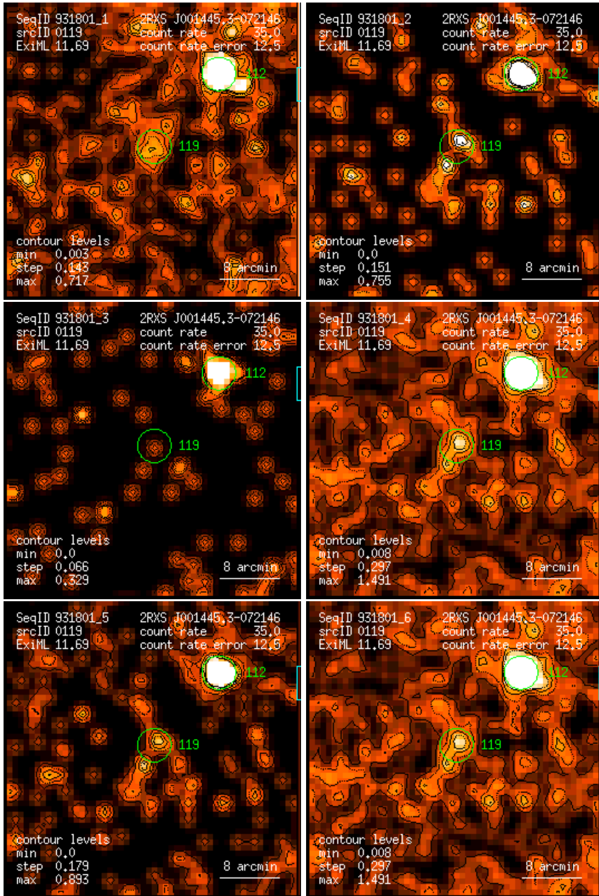
Figure 119: RASS 931801: detection 0119: band rate images, Gaussian filter: (1) PSPC channels 11 – 41, (2) 52 – 90, (3) 91 – 201, (4) 11 – 235, (5) 52 – 201, (6) 11 – 201. Broad band rates in counts/ks. Band rate contour levels in counts/ks/arcmin 2 .
