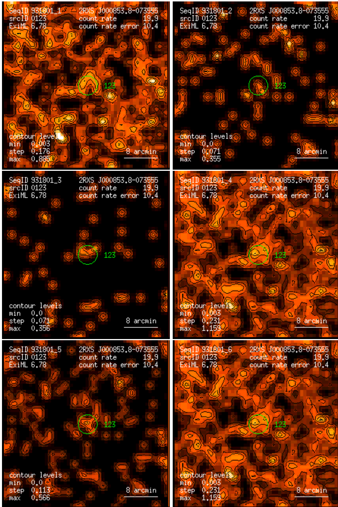
Figure 123: RASS 931801: detection 0123: band rate images, Gaussian filter: (1) PSPC channels 11 – 41, (2) 52 – 90, (3) 91 – 201, (4) 11 – 235, (5) 52 – 201, (6) 11 – 201. Broad band rates in counts/ks. Band rate contour levels in counts/ks/arcmin 2 .
