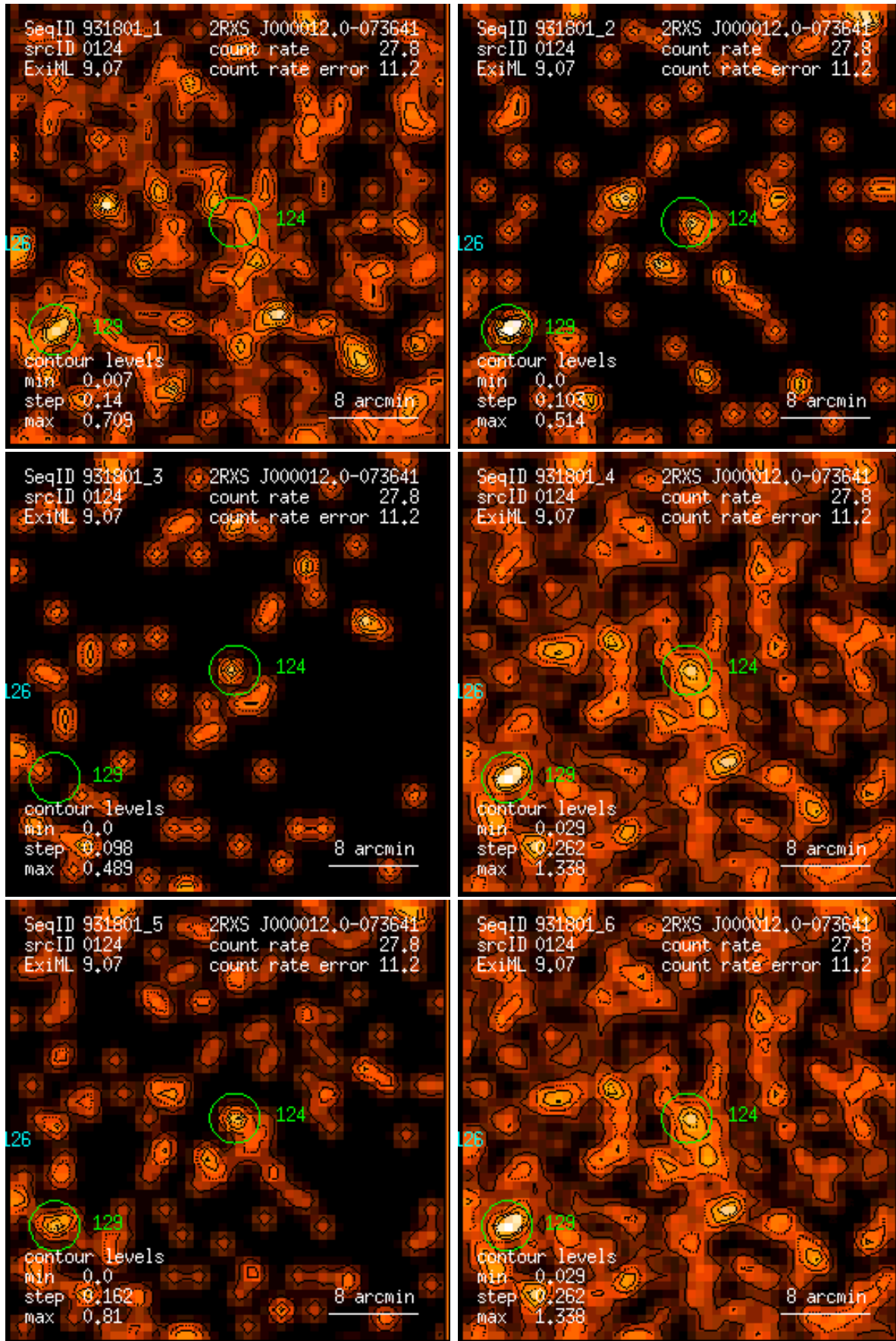
Figure 124: RASS 931801: detection 0124: band rate images, Gaussian filter: (1) PSPC channels 11 – 41, (2) 52 – 90, (3) 91 – 201, (4) 11 – 235, (5) 52 – 201, (6) 11 – 201. Broad band rates in counts/ks. Band rate contour levels in counts/ks/arcmin 2 .
