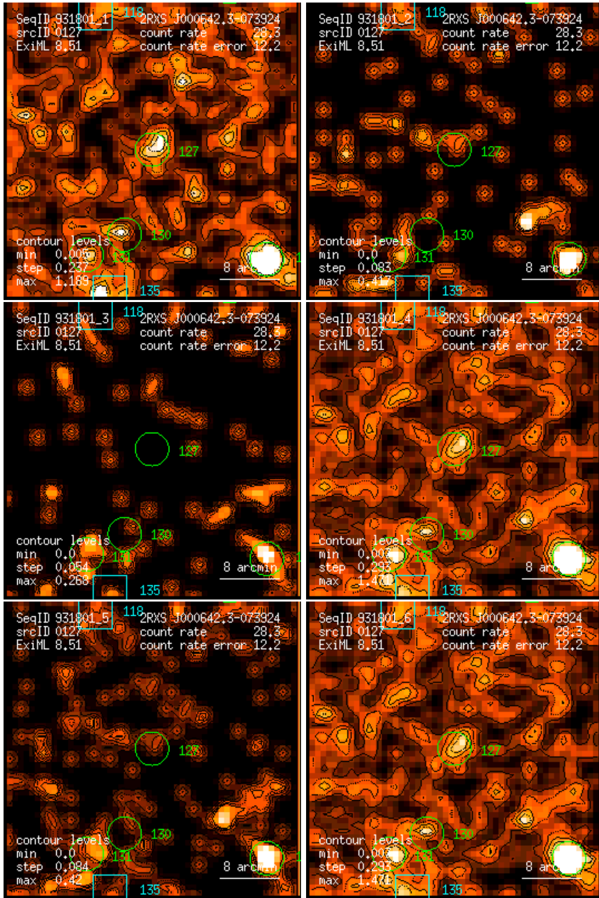
Figure 127: RASS 931801: detection 0127: band rate images, Gaussian filter: (1) PSPC channels 11 – 41, (2) 52 – 90, (3) 91 – 201, (4) 11 – 235, (5) 52 – 201, (6) 11 – 201. Broad band rates in counts/ks. Band rate contour levels in counts/ks/arcmin 2 .
