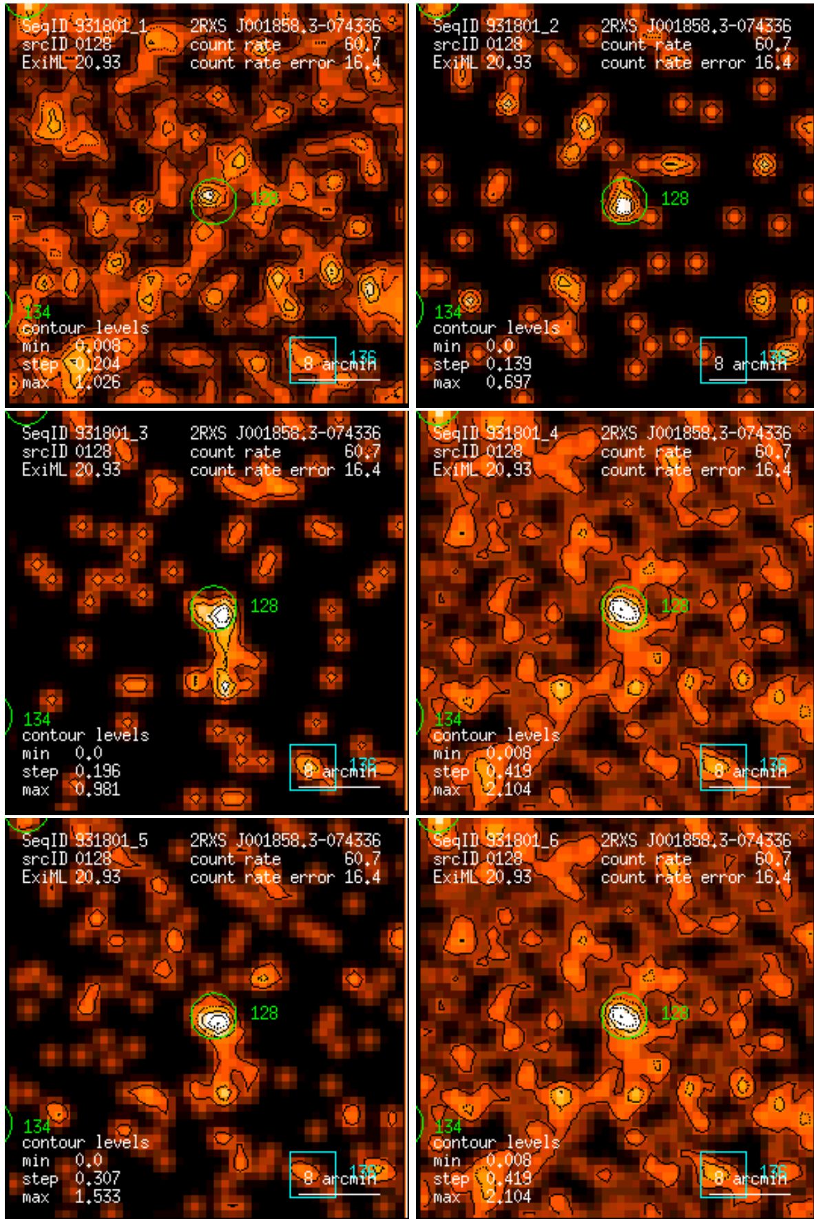
Figure 128: RASS 931801: detection 0128: band rate images, Gaussian filter: (1) PSPC channels 11 – 41, (2) 52 – 90, (3) 91 – 201, (4) 11 – 235, (5) 52 – 201, (6) 11 – 201. Broad band rates in counts/ks. Band rate contour levels in counts/ks/arcmin 2 .
