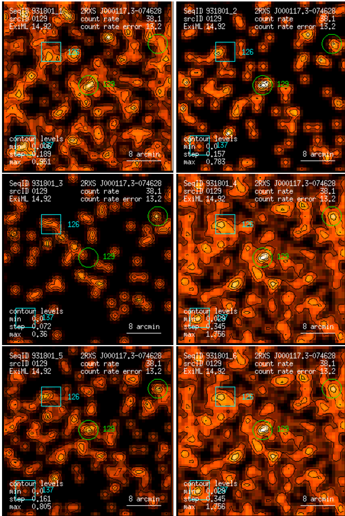
Figure 129: RASS 931801: detection 0129: band rate images, Gaussian filter: (1) PSPC channels 11 – 41, (2) 52 – 90, (3) 91 – 201, (4) 11 – 235, (5) 52 – 201, (6) 11 – 201. Broad band rates in counts/ks. Band rate contour levels in counts/ks/arcmin 2 .
