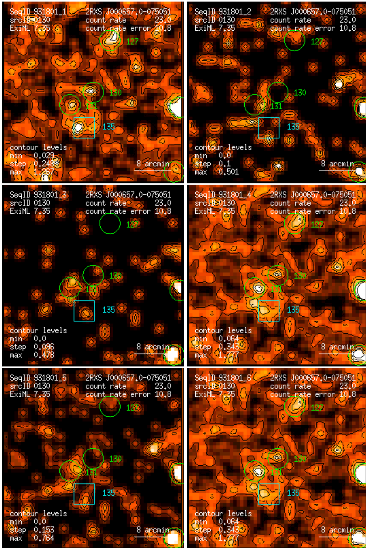
Figure 130: RASS 931801: detection 0130: band rate images, Gaussian filter: (1) PSPC channels 11 – 41, (2) 52 – 90, (3) 91 – 201, (4) 11 – 235, (5) 52 – 201, (6) 11 – 201. Broad band rates in counts/ks. Band rate contour levels in counts/ks/arcmin 2 .
