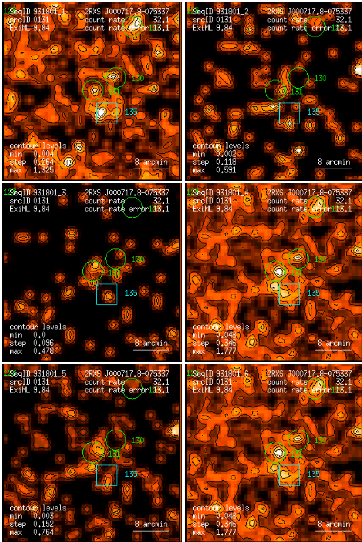
Figure 131: RASS 931801: detection 0131: band rate images, Gaussian filter: (1) PSPC channels 11 – 41, (2) 52 – 90, (3) 91 – 201, (4) 11 – 235, (5) 52 – 201, (6) 11 – 201. Broad band rates in counts/ks. Band rate contour levels in counts/ks/arcmin 2 .
