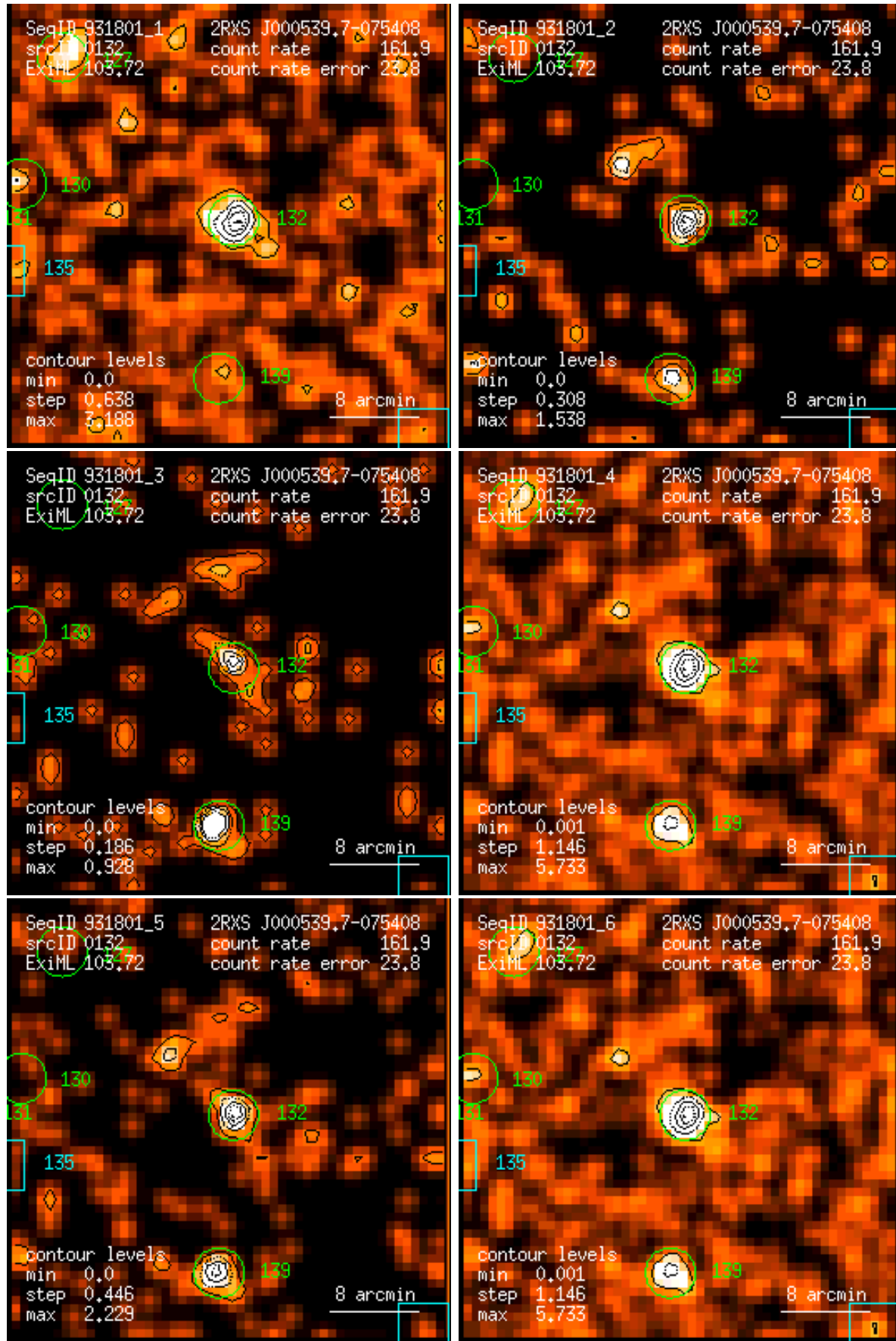
Figure 132: RASS 931801: detection 0132: band rate images, Gaussian filter: (1) PSPC channels 11 – 41, (2) 52 – 90, (3) 91 – 201, (4) 11 – 235, (5) 52 – 201, (6) 11 – 201. Broad band rates in counts/ks. Band rate contour levels in counts/ks/arcmin 2 .
