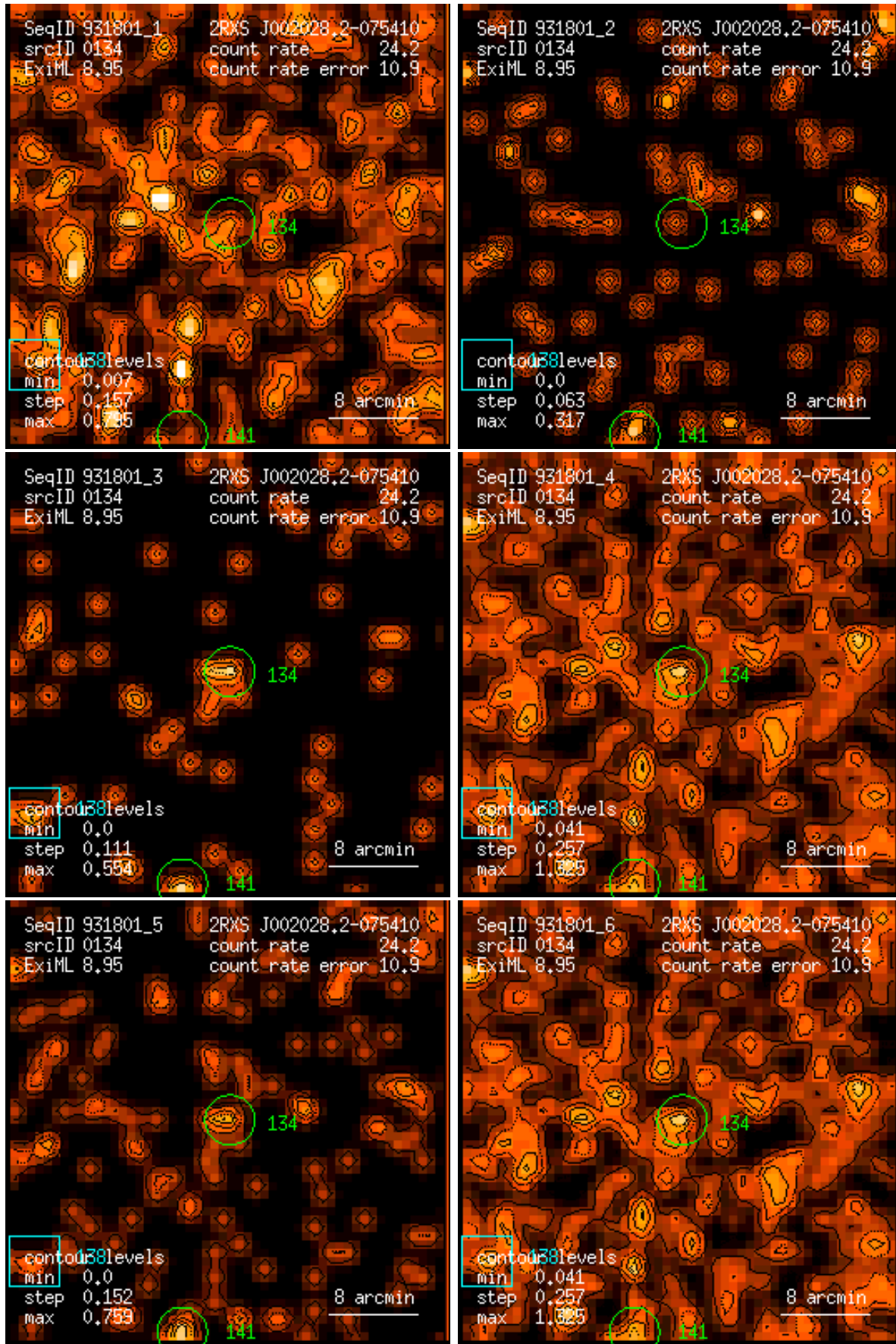
Figure 134: RASS 931801: detection 0134: band rate images, Gaussian filter: (1) PSPC channels 11 – 41, (2) 52 – 90, (3) 91 – 201, (4) 11 – 235, (5) 52 – 201, (6) 11 – 201. Broad band rates in counts/ks. Band rate contour levels in counts/ks/arcmin 2 .
