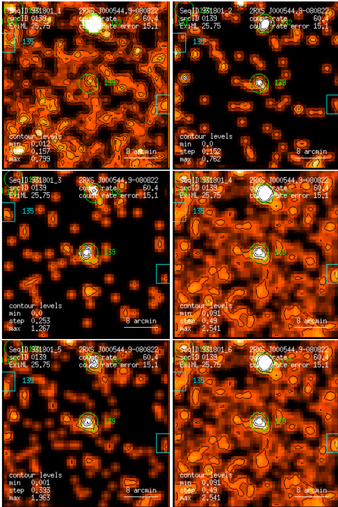
Figure 139: RASS 931801: detection 0139: band rate images, Gaussian filter: (1) PSPC channels 11 – 41, (2) 52 – 90, (3) 91 – 201, (4) 11 – 235, (5) 52 – 201, (6) 11 – 201. Broad band rates in counts/ks. Band rate contour levels in counts/ks/arcmin 2 .
