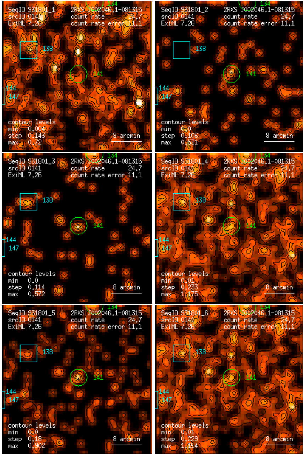
Figure 141: RASS 931801: detection 0141: band rate images, Gaussian filter: (1) PSPC channels 11 – 41, (2) 52 – 90, (3) 91 – 201, (4) 11 – 235, (5) 52 – 201, (6) 11 – 201. Broad band rates in counts/ks. Band rate contour levels in counts/ks/arcmin 2 .
