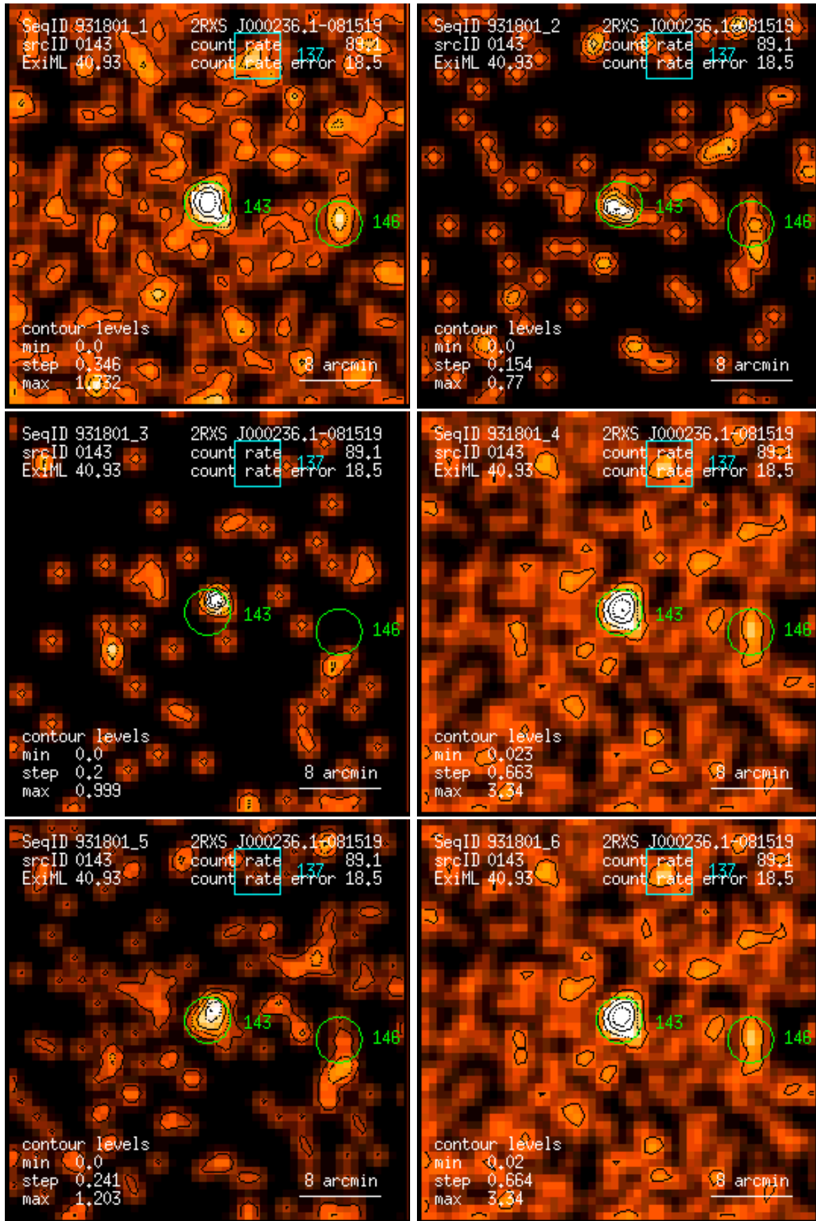
Figure 143: RASS 931801: detection 0143: band rate images, Gaussian filter: (1) PSPC channels 11 – 41, (2) 52 – 90, (3) 91 – 201, (4) 11 – 235, (5) 52 – 201, (6) 11 – 201. Broad band rates in counts/ks. Band rate contour levels in counts/ks/arcmin 2 .
