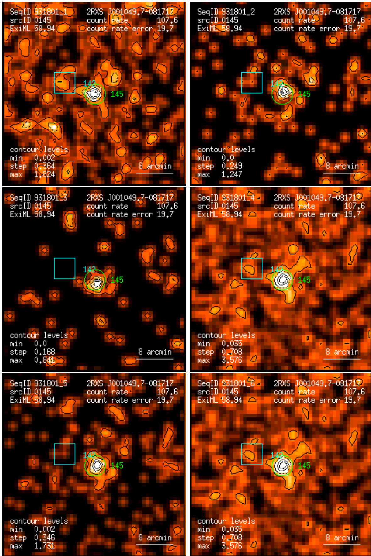
Figure 145: RASS 931801: detection 0145: band rate images, Gaussian filter: (1) PSPC channels 11 – 41, (2) 52 – 90, (3) 91 – 201, (4) 11 – 235, (5) 52 – 201, (6) 11 – 201. Broad band rates in counts/ks. Band rate contour levels in counts/ks/arcmin 2 .
