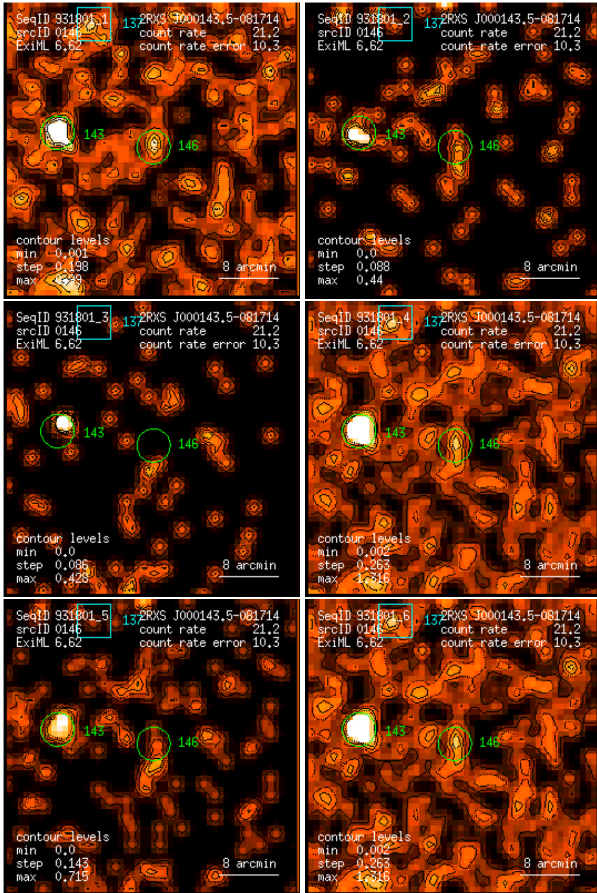
Figure 146: RASS 931801: detection 0146: band rate images, Gaussian filter: (1) PSPC channels 11 – 41, (2) 52 – 90, (3) 91 – 201, (4) 11 – 235, (5) 52 – 201, (6) 11 – 201. Broad band rates in counts/ks. Band rate contour levels in counts/ks/arcmin 2 .
