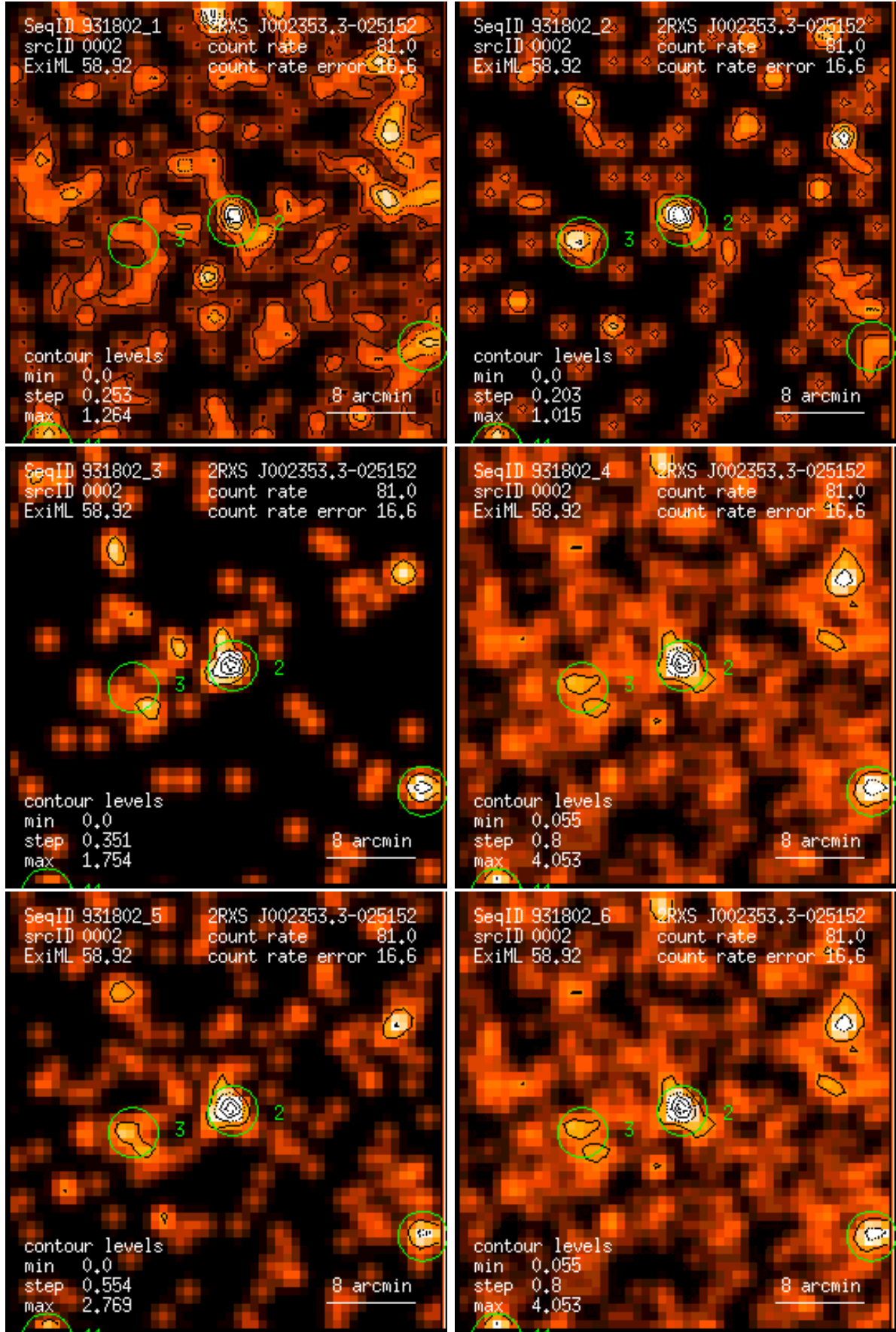
Figure 2: RASS 931802: detection 0002: band rate images, Gaussian filter: (1) PSPC channels 11 – 41, (2) 52 – 90, (3) 91 – 201, (4) 11 – 235, (5) 52 – 201, (6) 11 – 201. Broad band rates in counts/ks. Band rate contour levels in counts/ks/arcmin 2 .
