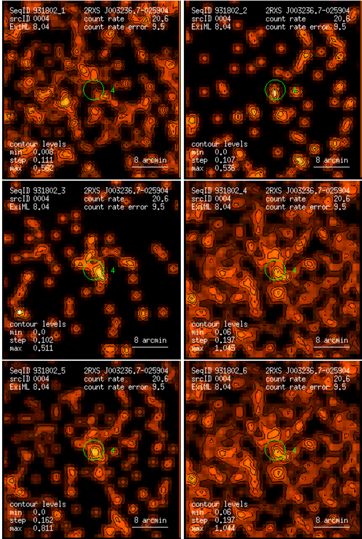
Figure 4: RASS 931802: detection 0004: band rate images, Gaussian filter: (1) PSPC channels 11 – 41, (2) 52 – 90, (3) 91 – 201, (4) 11 – 235, (5) 52 – 201, (6) 11 – 201. Broad band rates in counts/ks. Band rate contour levels in counts/ks/arcmin 2 .
