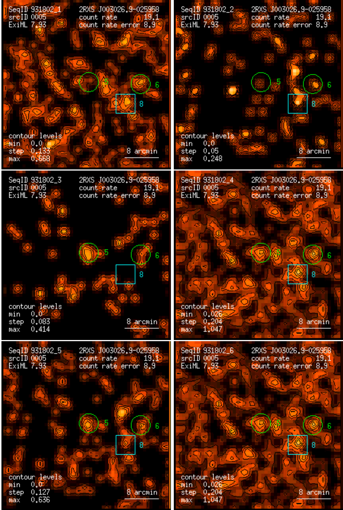
Figure 5: RASS 931802: detection 0005: band rate images, Gaussian filter: (1) PSPC channels 11 – 41, (2) 52 – 90, (3) 91 – 201, (4) 11 – 235, (5) 52 – 201, (6) 11 – 201. Broad band rates in counts/ks. Band rate contour levels in counts/ks/arcmin 2 .
