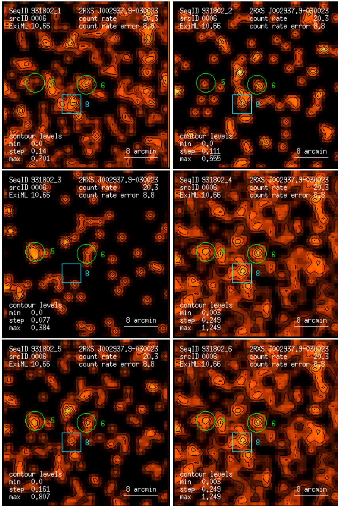
Figure 6: RASS 931802: detection 0006: band rate images, Gaussian filter: (1) PSPC channels 11 – 41, (2) 52 – 90, (3) 91 – 201, (4) 11 – 235, (5) 52 – 201, (6) 11 – 201. Broad band rates in counts/ks. Band rate contour levels in counts/ks/arcmin 2 .
