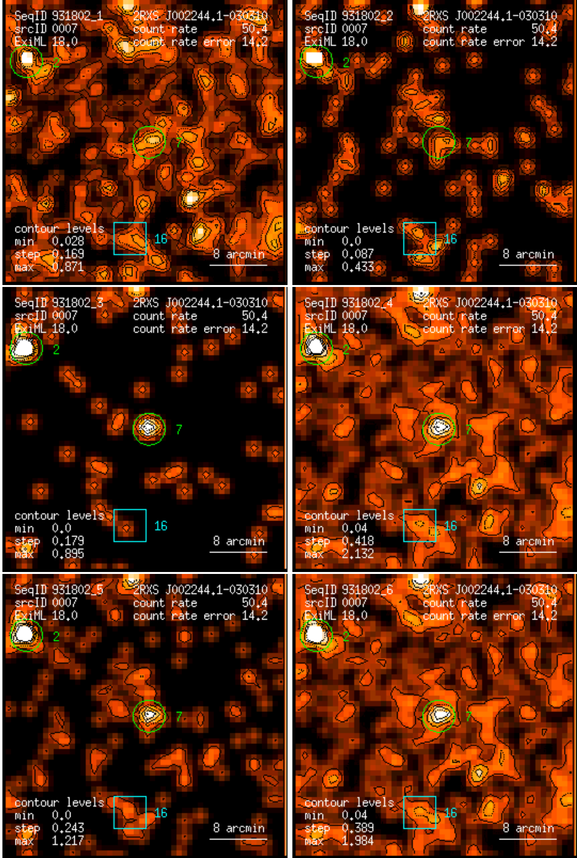
Figure 7: RASS 931802: detection 0007: band rate images, Gaussian filter: (1) PSPC channels 11 – 41, (2) 52 – 90, (3) 91 – 201, (4) 11 – 235, (5) 52 – 201, (6) 11 – 201. Broad band rates in counts/ks. Band rate contour levels in counts/ks/arcmin 2 .
